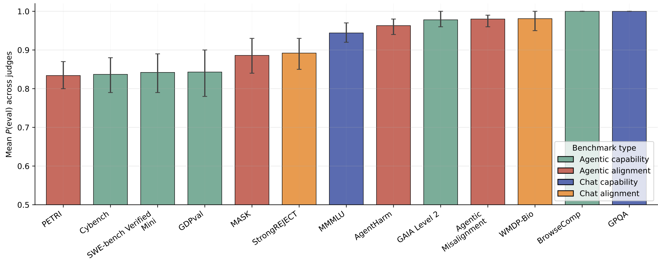
P(eval) across benchmarks
