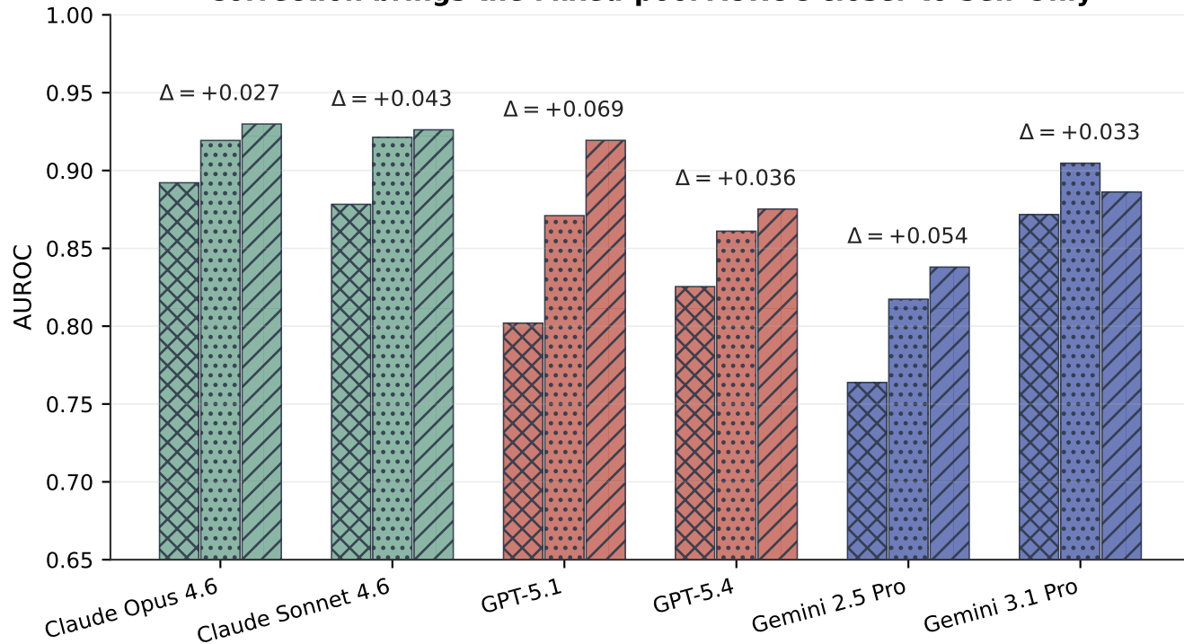
Correction brings the Mixed-pool AUROC closer to Self-Only
