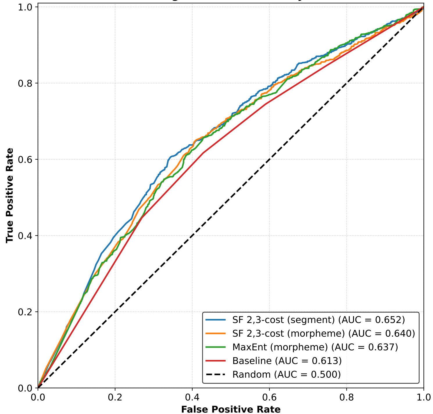
Item-Weighted ROC Curves by Model
