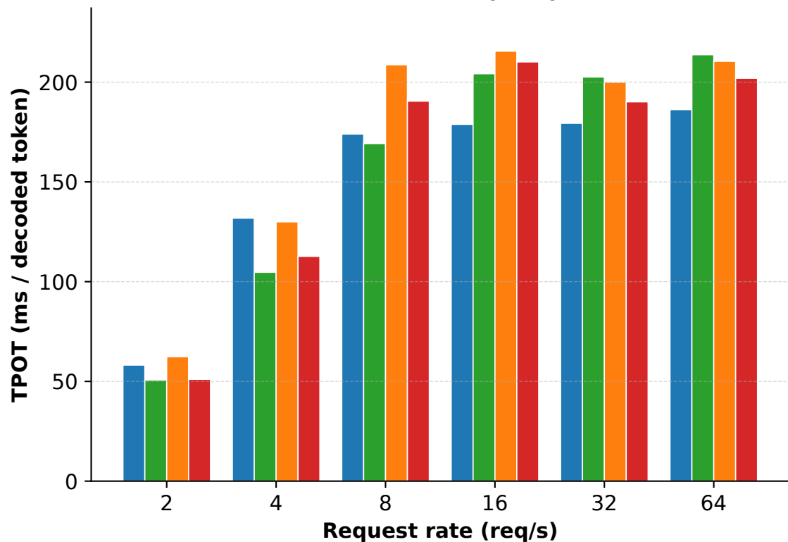
Mean TPOT (raw)
