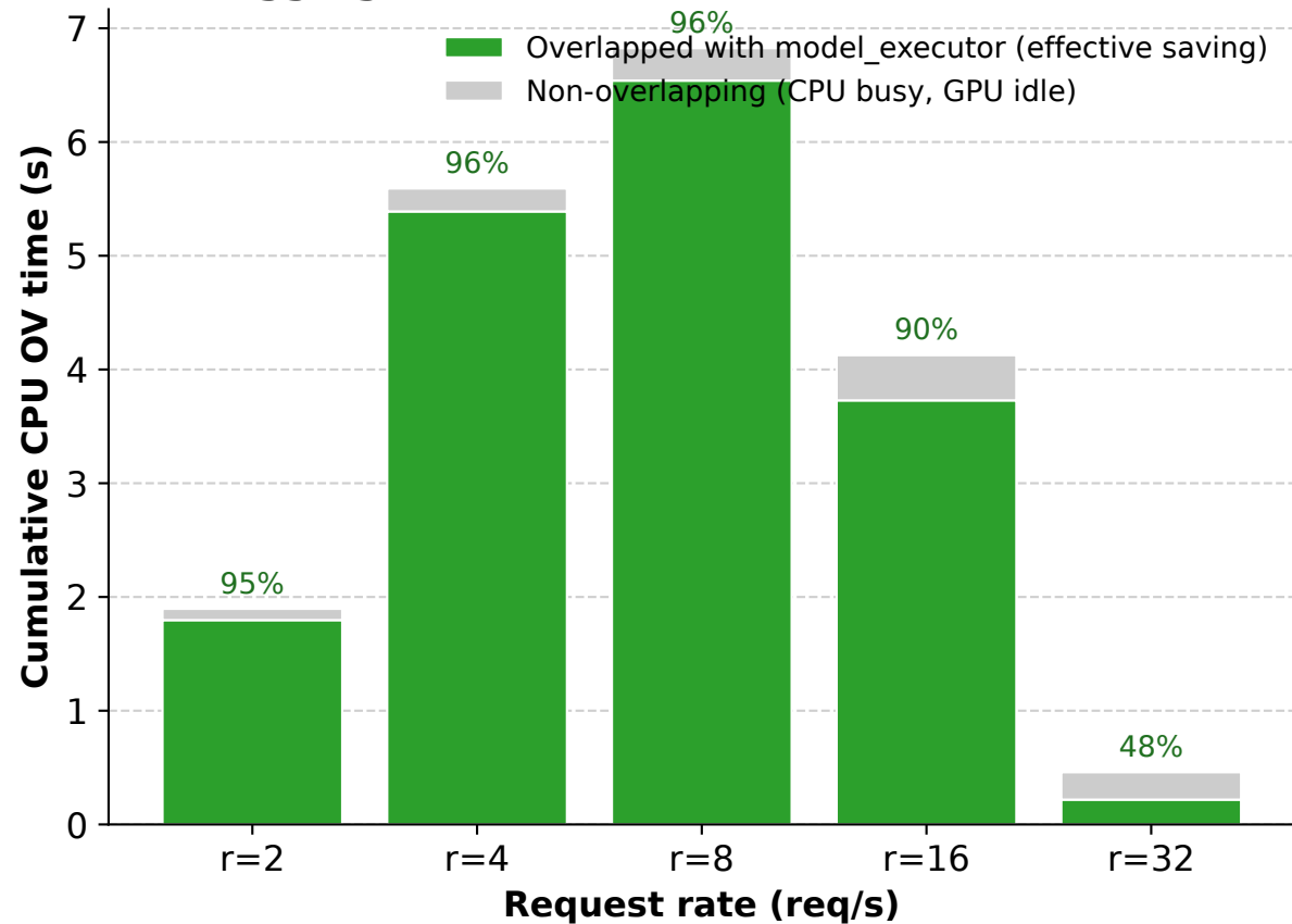
Aggregate: effective vs wasted CPU OV time
