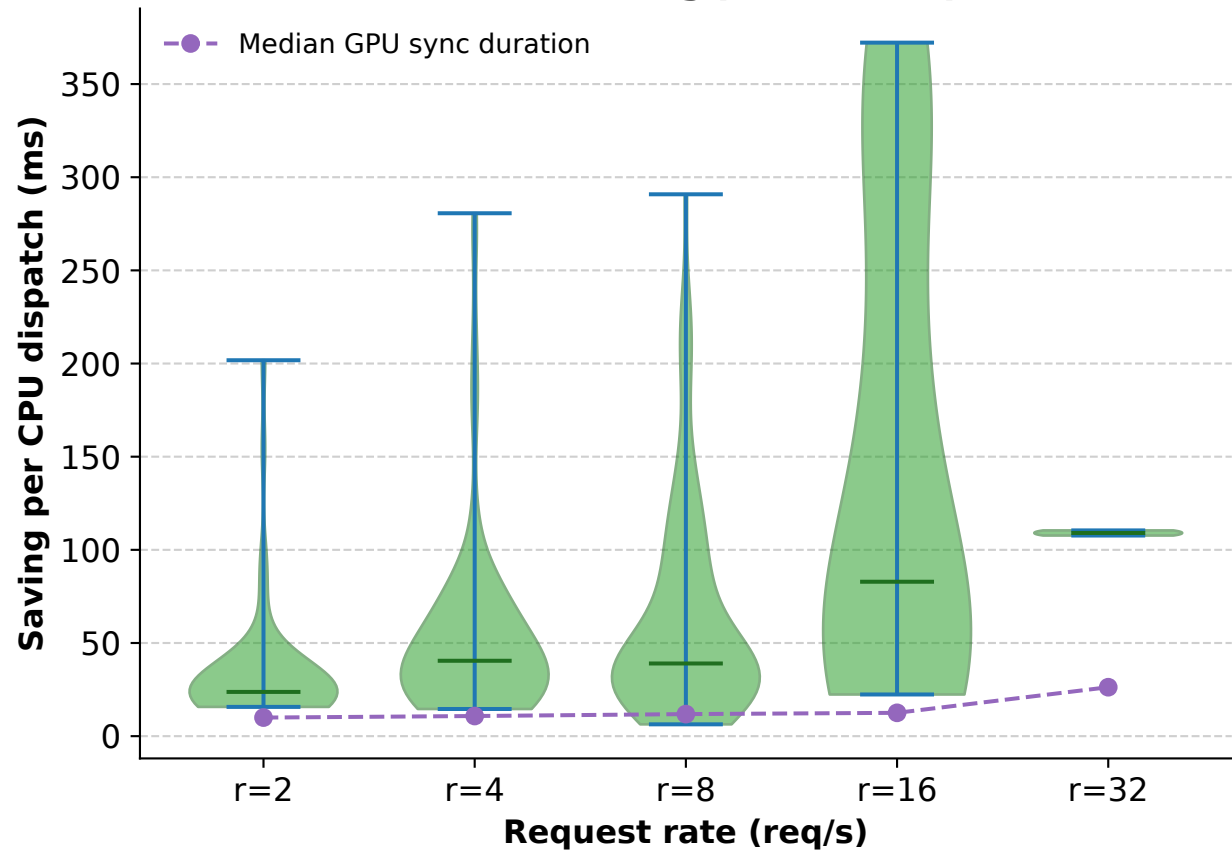
Distribution: saving per CPU dispatch
