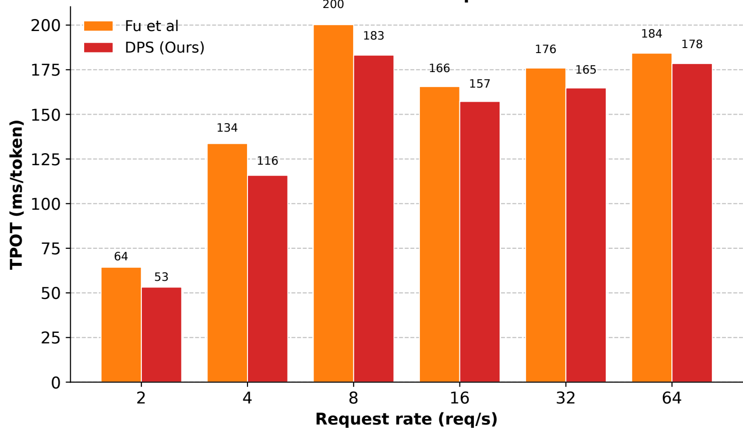
Median Time-Per-Output-Token
