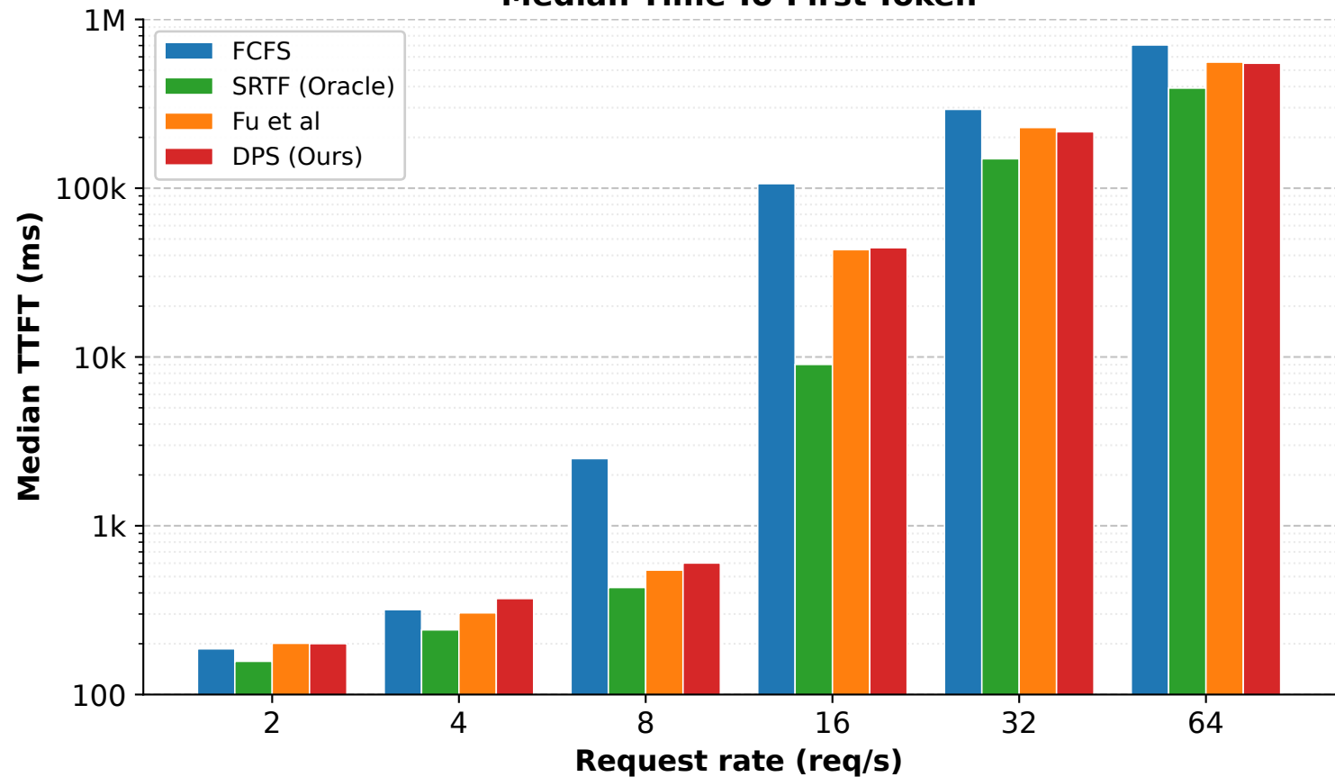
Median Time-To-First-Token
