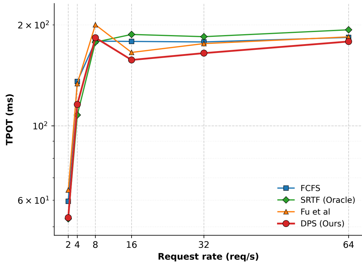
Median TPOT
