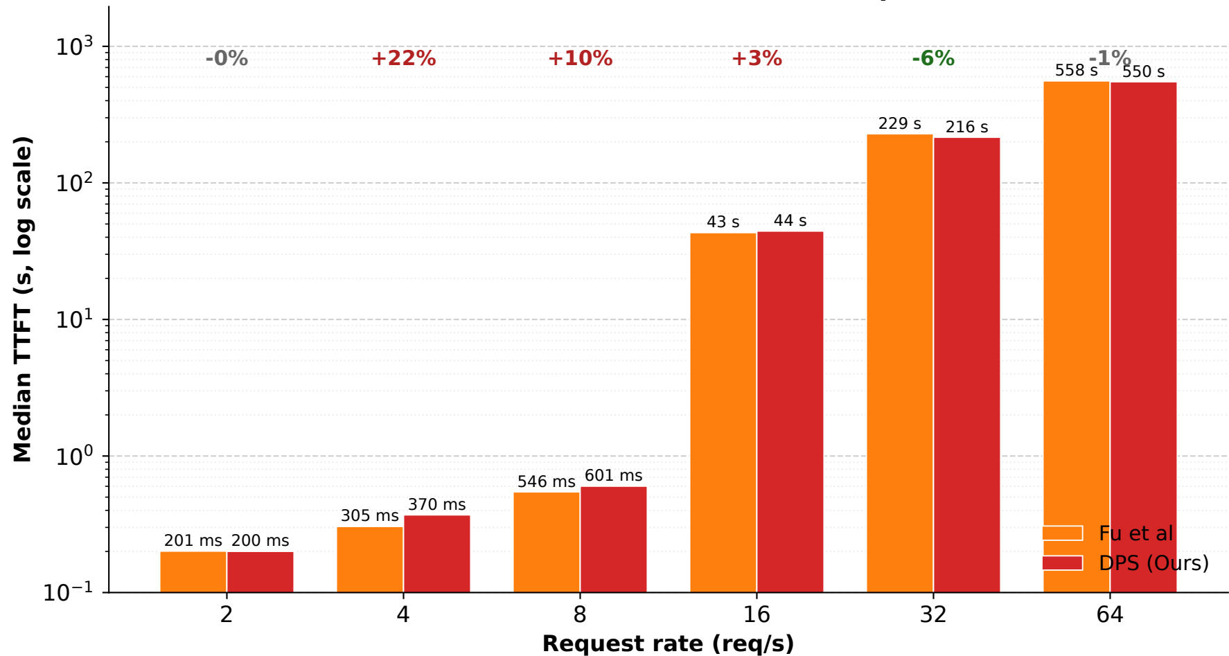
Median TTFT — DPS vs Fu et al. across request rates
