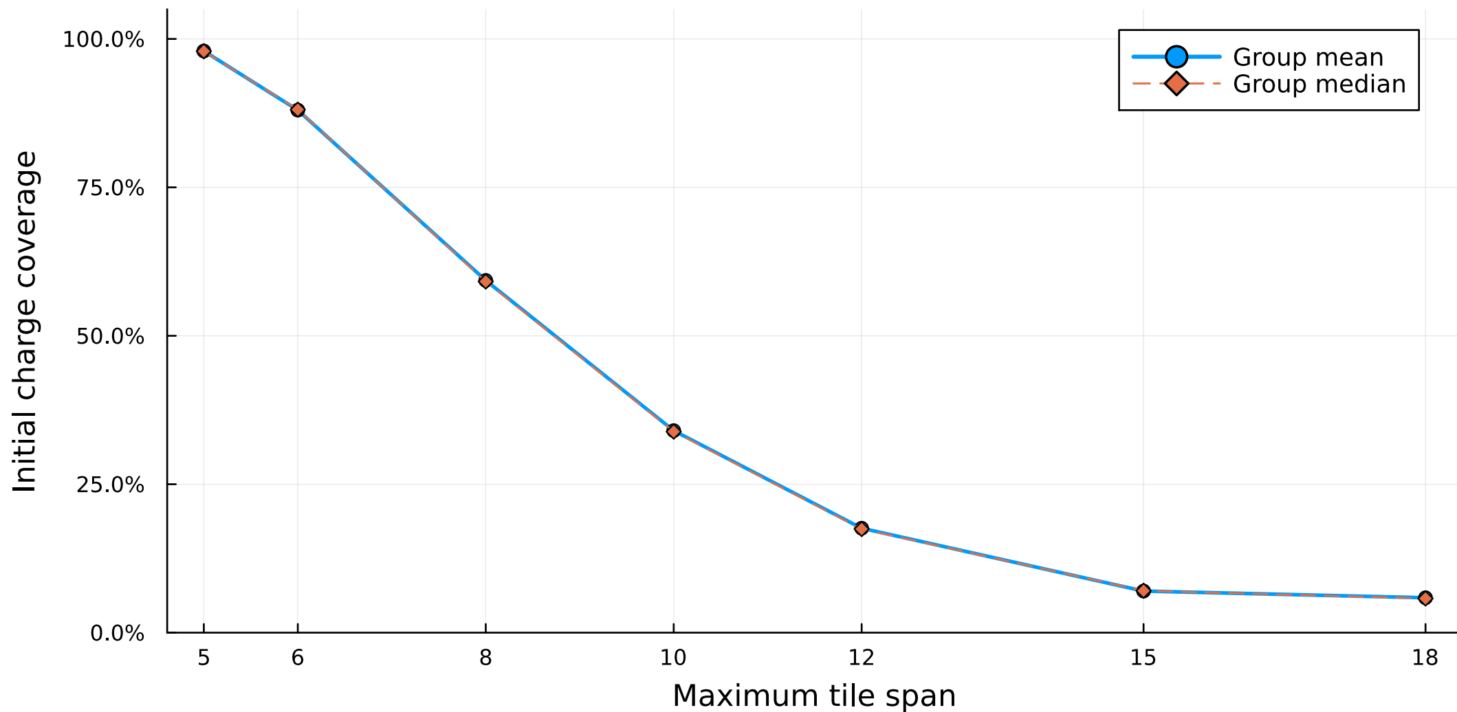
Coverage of full-indicator charges by 500 uniform initial samples
