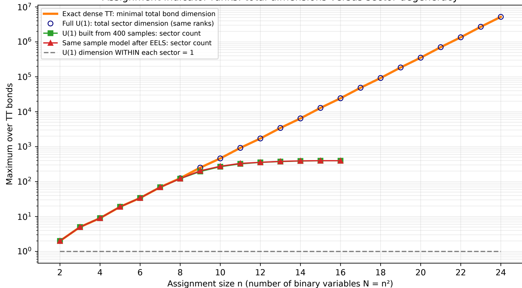
Assignment indicator ranks: total dimensions versus sector degeneracy
