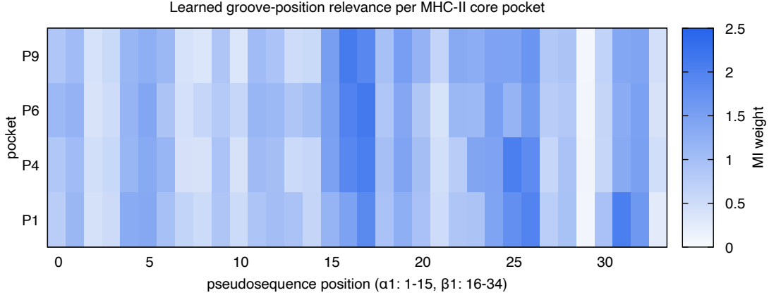
Figure 2: Learned mutual-information relevance w_{j,p} of each groove pseudosequence position p ( x ) for each MHC-II core pocket j (rows), over human class-II alleles. Relevance concentrates on the polymorphic \beta_1 region; different pockets emphasize different positions. bench/make_figures.py .
