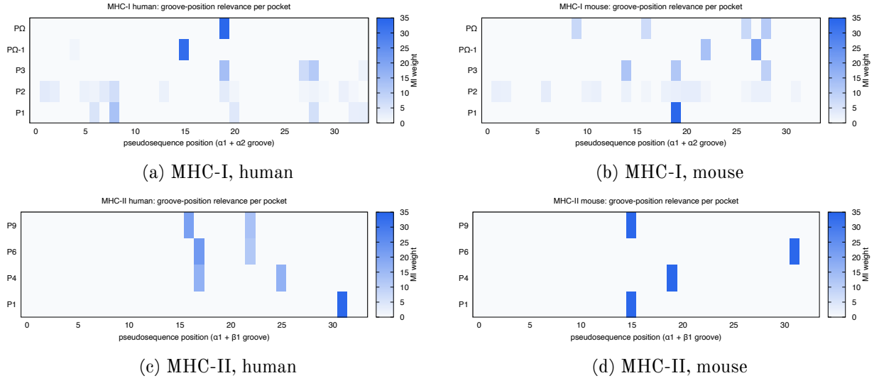
Figure 5: DPI-pruned mutual-information relevance w_{j,p} of each groove pseudosequence position p ( x ) for each anchor pocket j (rows), per class and species. After data-processing-inequality pruning [12] each pocket keeps only its direct positions (MHC-I P \Omega \rightarrow \sim 19 , P2 \rightarrow \sim 7-8 , disjoint); MHC-II concentrates on \beta_1 . bench/make_figures.py .
