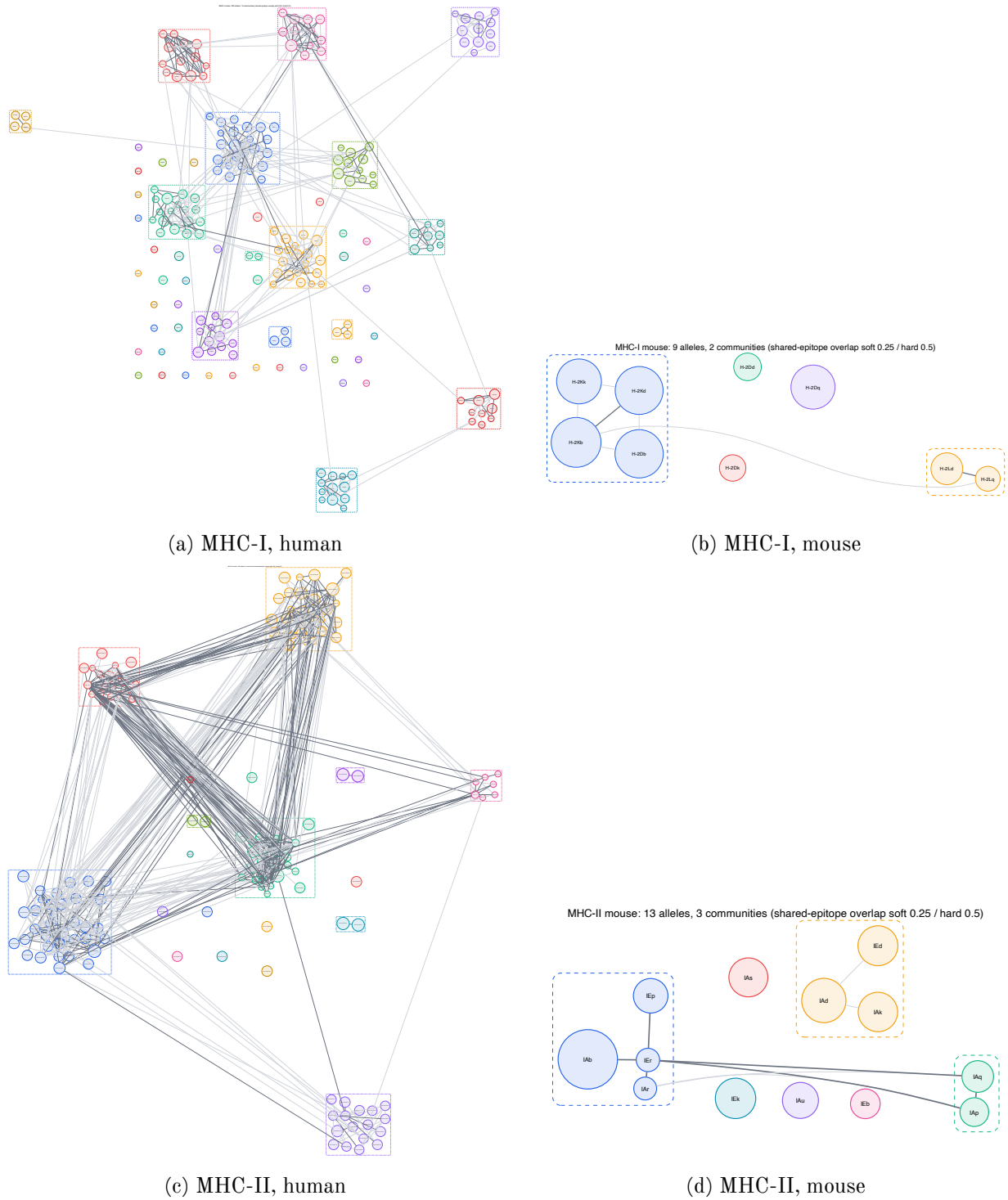
Figure 4: Observed co-presentation networks (shared-epitope overlap coefficient; thin \geq 0.25 , bold \geq 0.5 ; greedy-modularity communities), all four class \times species panels. Communities are coarser than the predicted groove network (Fig. 3) because promiscuous peptides bridge supertypes. bench/promiscuity_graph.py .
