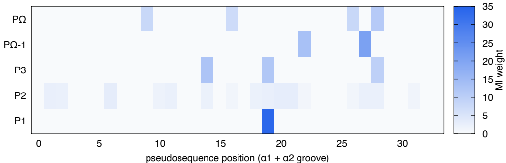
MHC-I mouse: groove-position relevance per pocket
