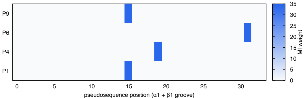
MHC-II mouse: groove-position relevance per pocket
