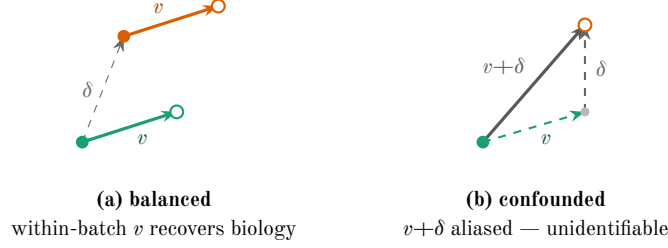
Figure 7: Batch cancellation needs a balanced design (Prop. 36, Rem. 6). (a) When both batches contain case and control, the case→control vector v (biology) is identical across batches while their absolute positions differ by the batch shift \delta , so a within-batch (paired) contrast recovers v free of \delta . (b) When batch is confounded with the phenotype — cases in one run, controls in another — the observed difference is v + \delta with no within-batch pair to split it (the true v and \delta , dashed, are unobservable): they are aliased and unidentifiable. Filled = case, open = control; teal = batch 1, orange = batch 2. Structure partly rescues (b) — \delta lives mainly in the V/J -usage and depth subspace, adjustable without unmixing the CDR3 signal (Rem. 6).
