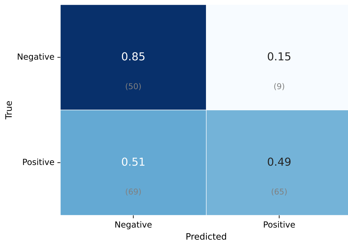
TRA (tcnnet) Precision: 0.878 • Recall: 0.485 • F1: 0.625
