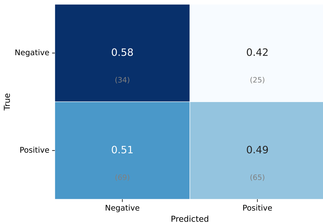
TRB only Precision: 0.722 • Recall: 0.485 • F1: 0.580
