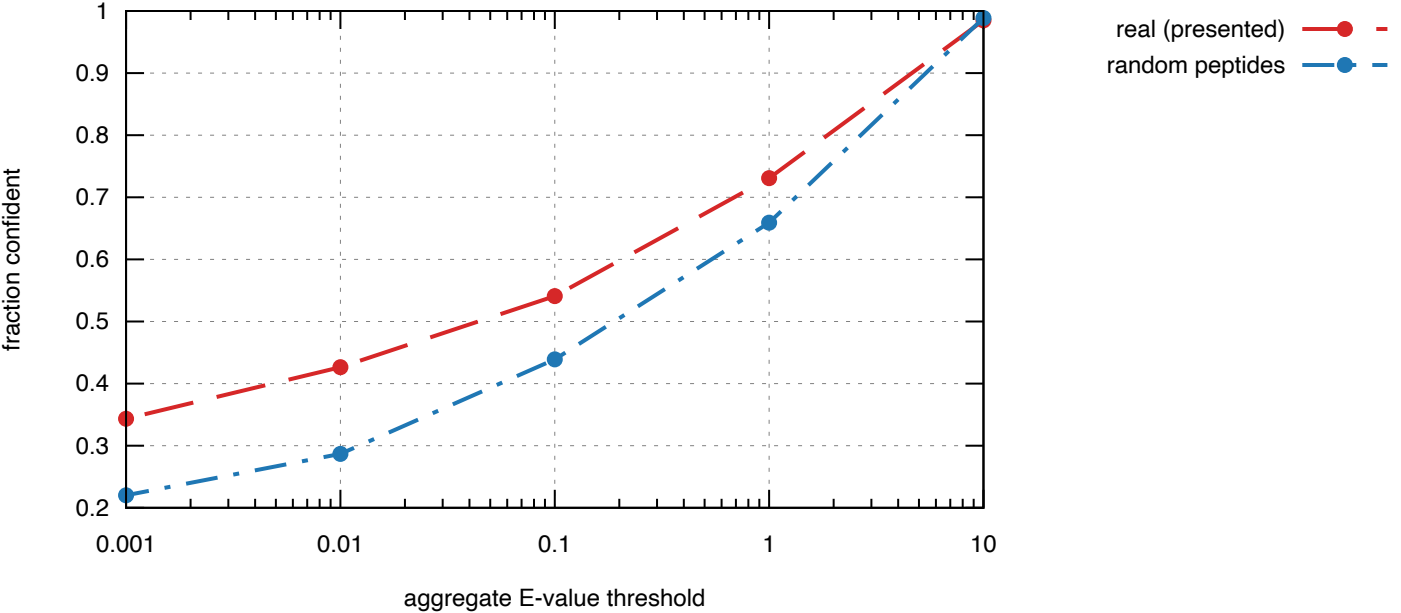
MHC class II: allele-guess confidence ( E \leq \text{thr} ), real vs random [top-1 acc 0.34, AUROC 0.58]
