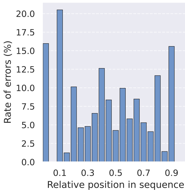
Classification error rate by positions in a sequence(%)
