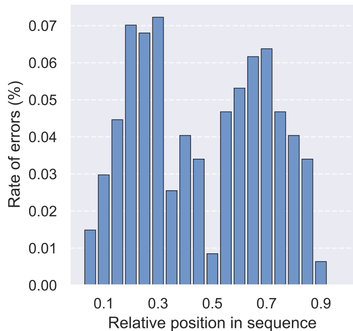
Classification error rate by positions in a sequence(%)
