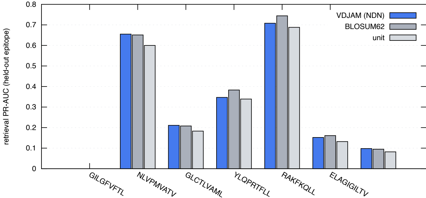
Leave-one-out-by-epitope retrieval (TRB, scope 2)
