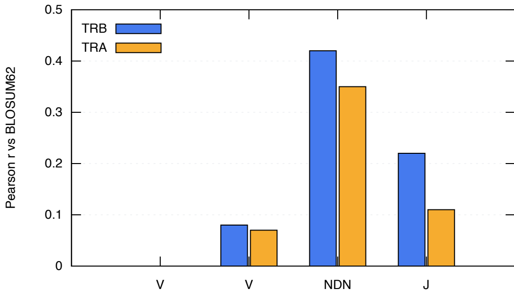
Substitution-matrix agreement with BLOSUM62 by CDR3 region
