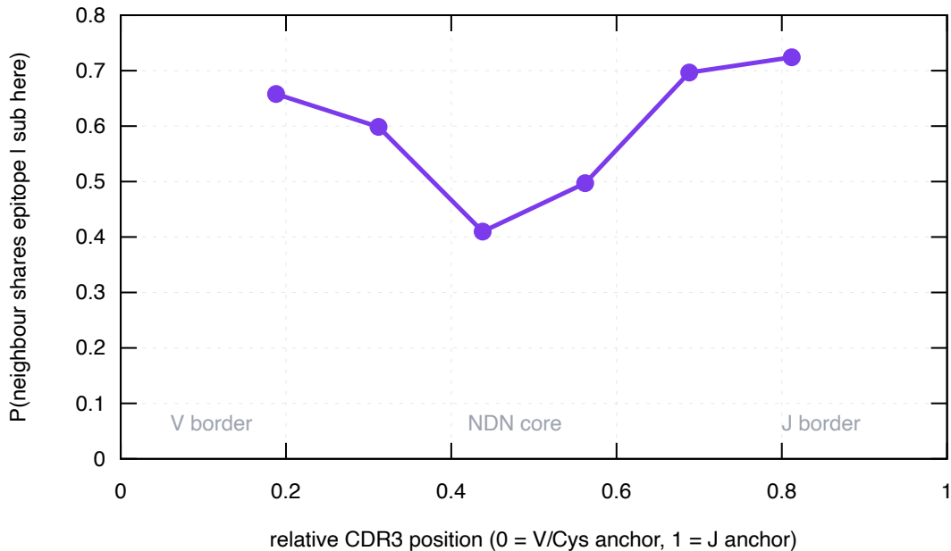
Single-substitution significance by CDR3 position (TRB)
