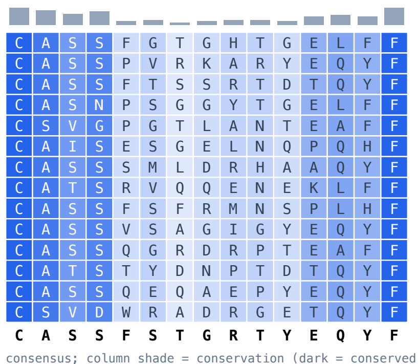
Figure 8: NLV (CMV pp65, A*02) TRB CDR3 block; same conservation pattern.
