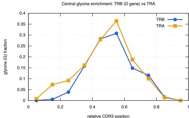
Figure 6: Glycine fraction by relative CDR 3 position: the NDN core is \sim 30\text{--}36\% glycine in both TRA and TRB (insertion/D-gene signature).
