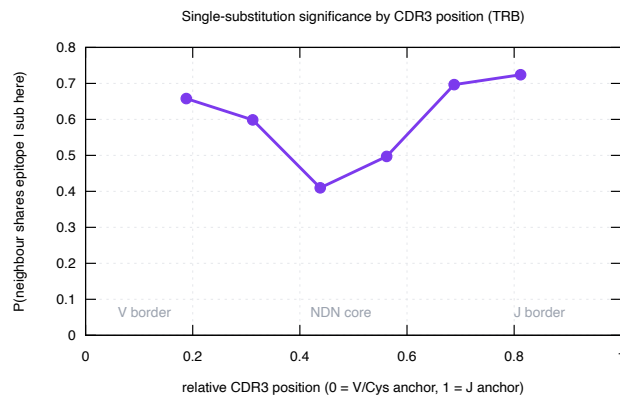
Figure 5: \Pr(\text{neighbour shares epitope} \mid \text{single substitution at relative position}) , TRB. The NDN core is where a mismatch most changes specificity; the V/J borders are germline noise.
