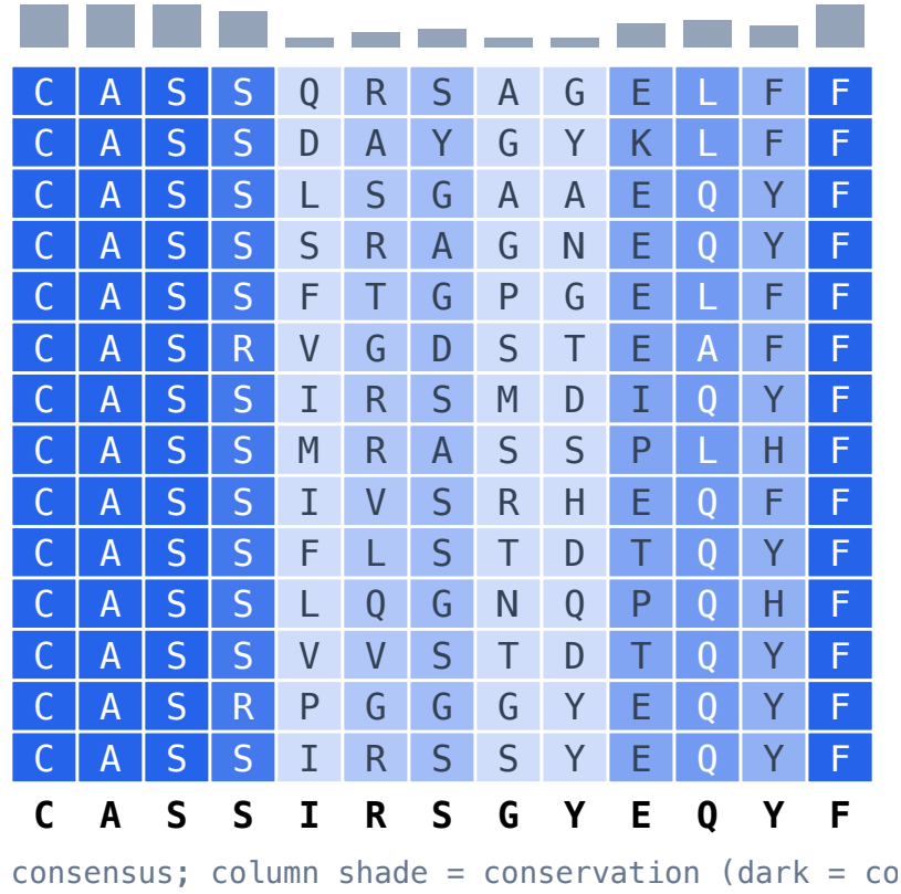
Figure 7: GIL (influenza M1, A*02) TRB CDR3 block; conserved V/J flanks, variable NDN core.
