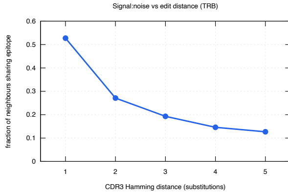
Figure 4: Fraction of CDR3 neighbours sharing an epitope vs Hamming distance (TRB): distance 1 is the signal:noise optimum [3].
