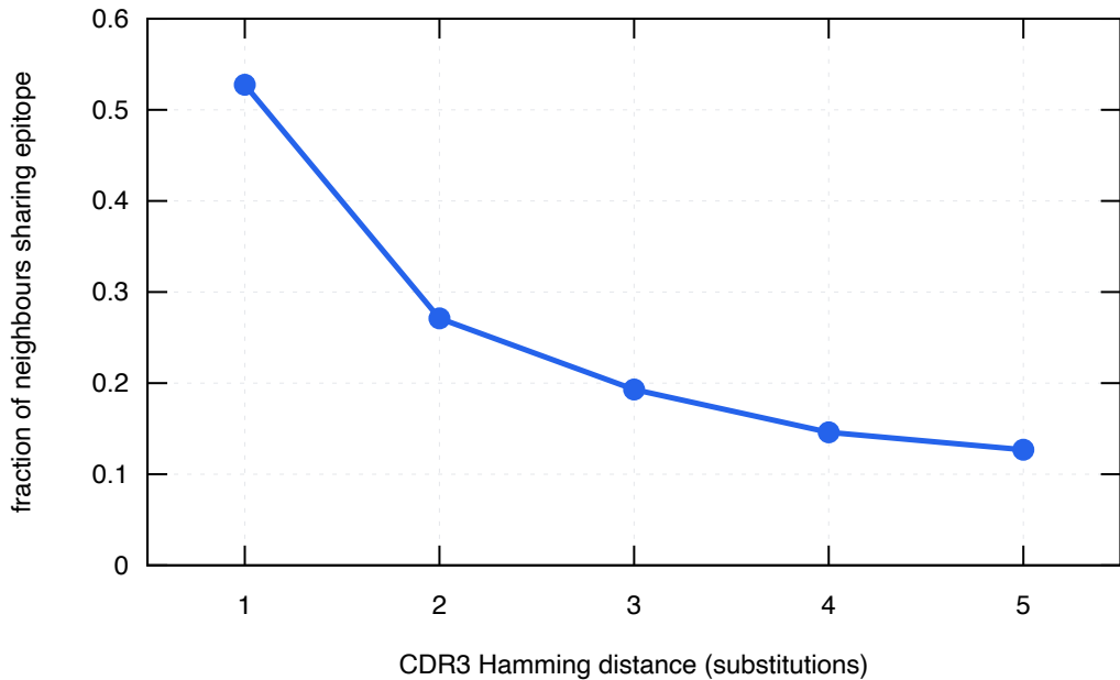
Signal:noise vs edit distance (human TRB)
