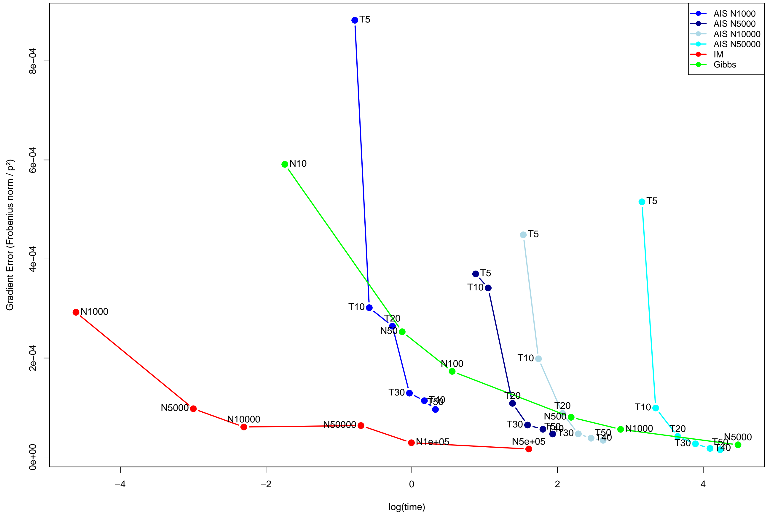
Gradient Error vs log(Time)
