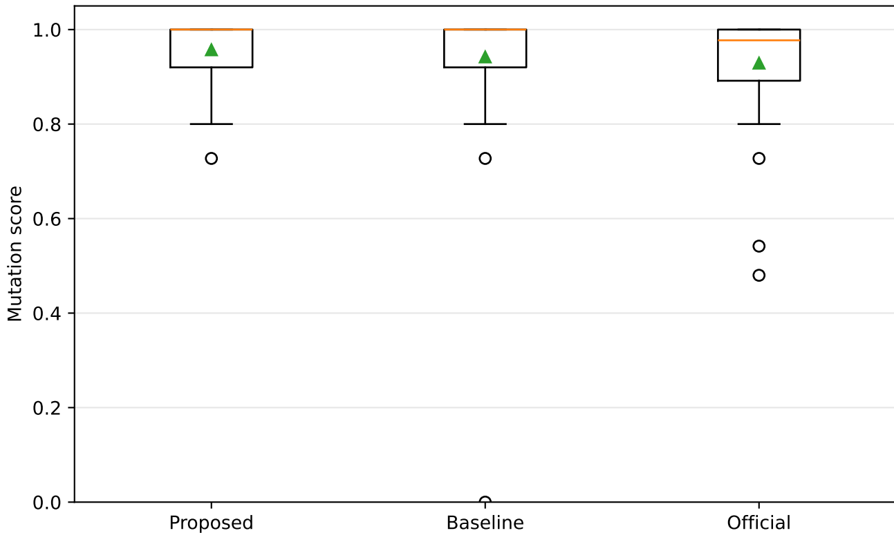
Task-level mutation score distribution
