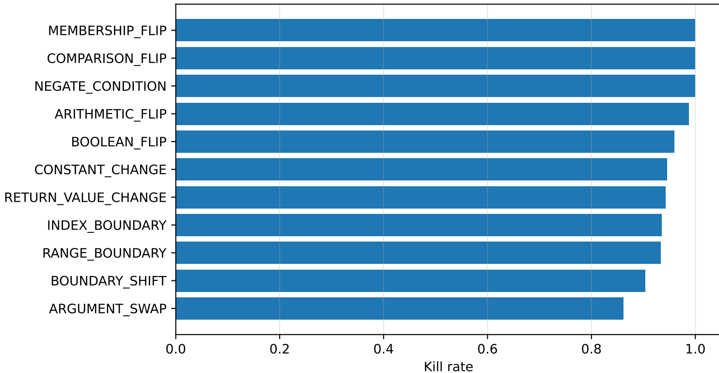
Mutation difficulty by operator
