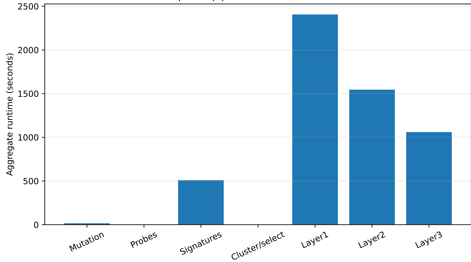
Proposed-pipeline runtime breakdown
