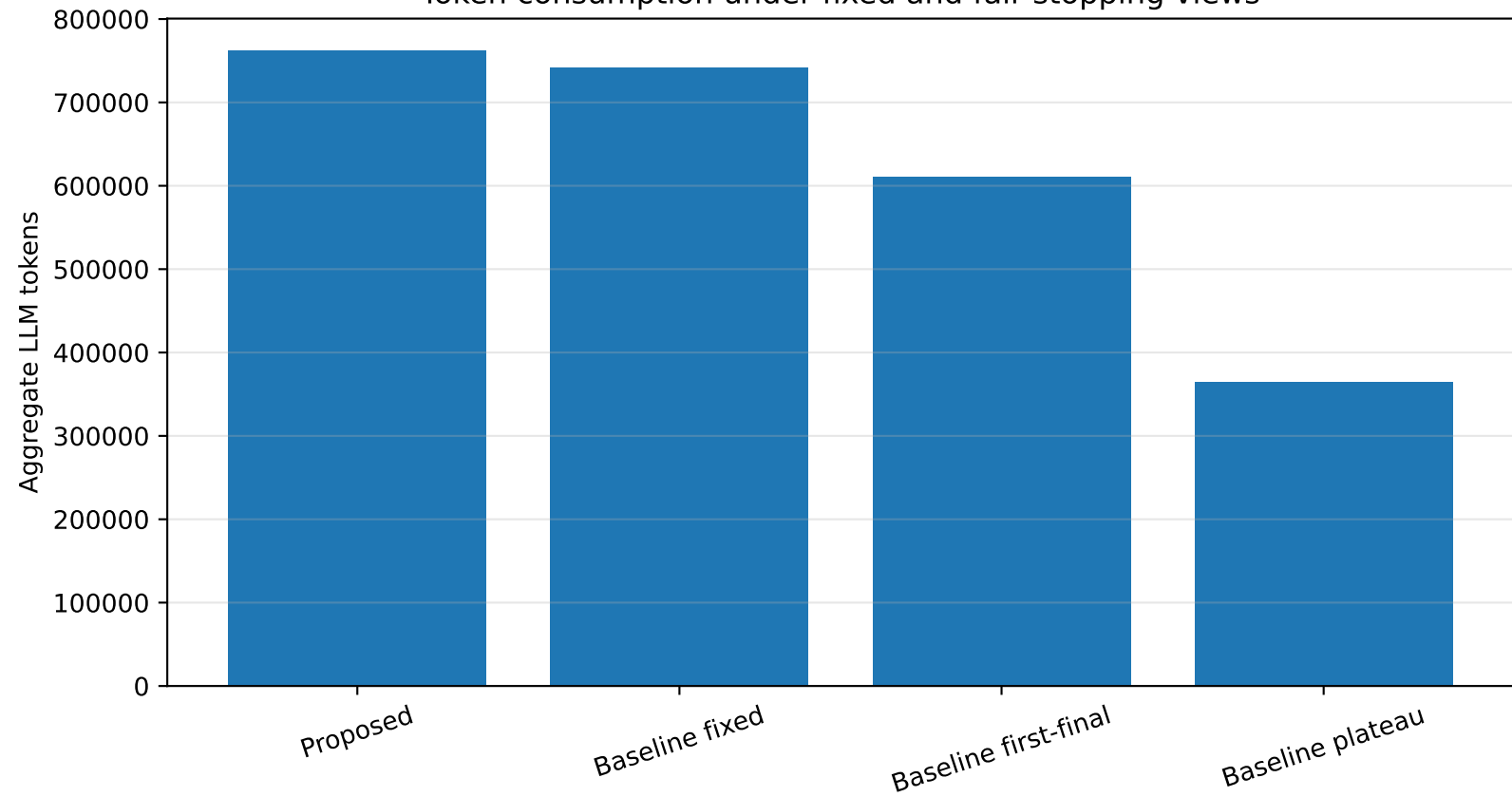
Token consumption under fixed and fair stopping views
