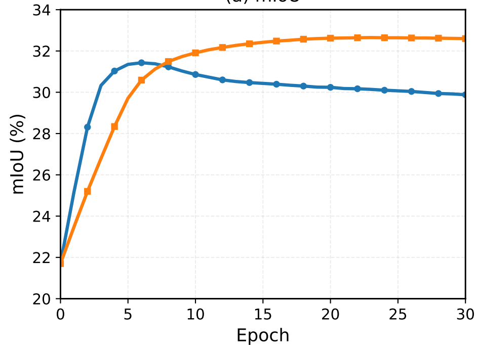
(a) mIoU
