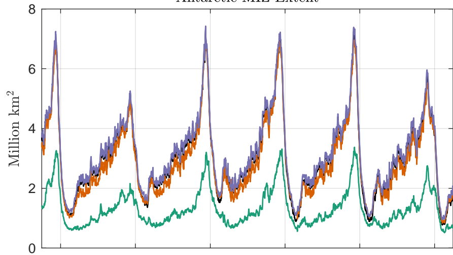
Antarctic MIZ Extent
