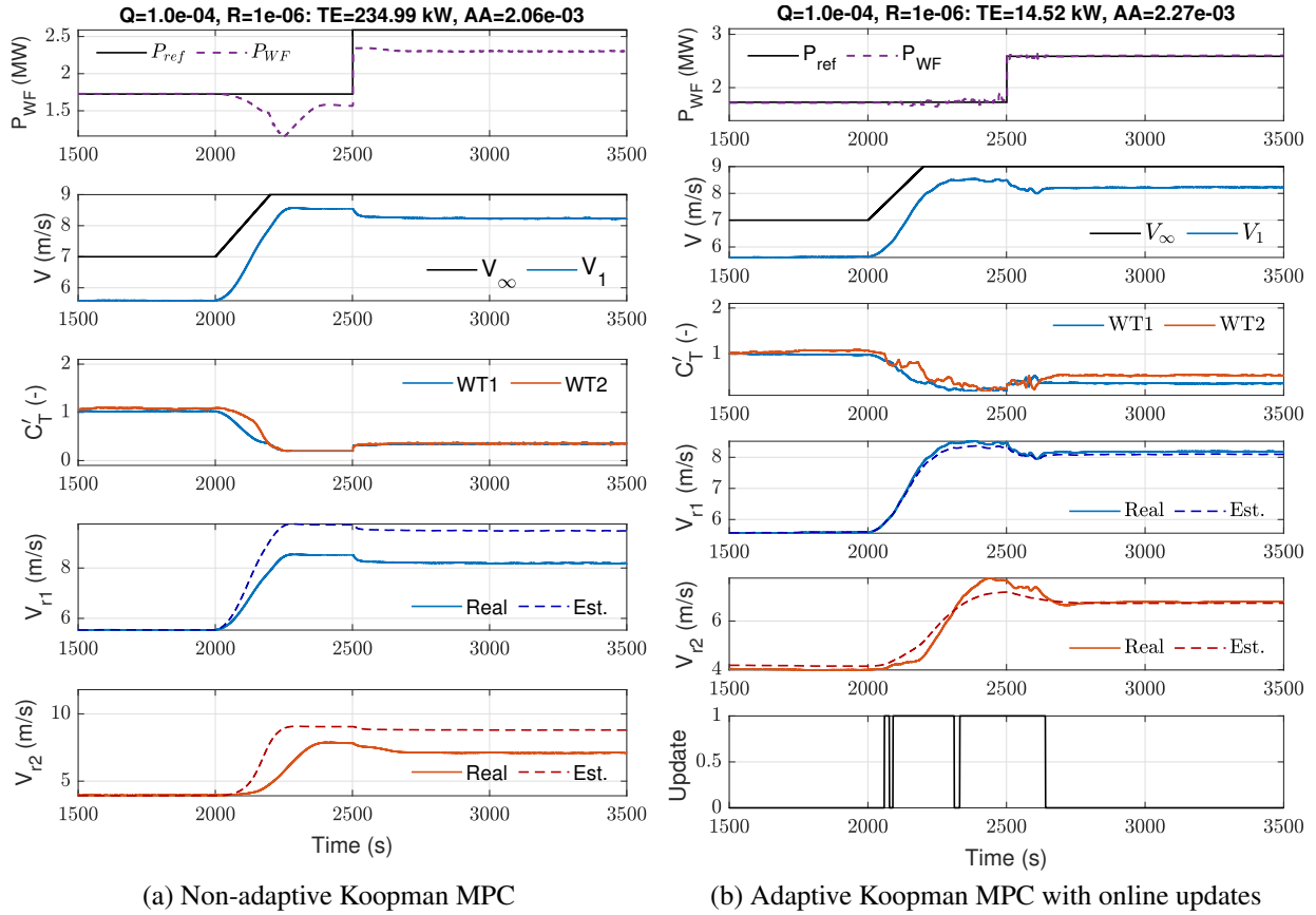
Figure 5.6: Closed-loop tracking comparison during a wind speed ramp and power reference step. Subplots (top to bottom): reference P_{ref} (black) and total power P_{WF} (purple dashed); wind speeds V_{\infty} (black) and V_1 (blue); thrust C_T ; and real vs. estimated effective wind V_{r1} , V_{r2} . Bottom plot in (b) shows the update signal (black). WT1/WT2 signals are blue/red; dashed lines denote estimates.
