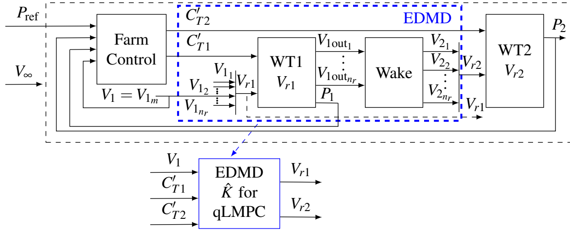
Figure 5.3: Block diagram of WFSim for AIC with farm control inputs P_{\text{ref}} , P_1 , P_2 , and V_1 = V_{1m} , thrust control signals C'_{T1} and C'_{T2} and freestream wind V_\infty . Wind speeds directly in front and behind the turbine WT1 are V_{11} to V_{1nr} and V_{1out1} to V_{1outnr} . Wind speeds directly in front of the turbine WT2 are V_{21} to V_{2nr} . The input to the EDMD model (dashed blue box in the closed-loop diagram and blue box below the diagram) are V_1 , C'_{T1} and C'_{T2} and its output are the effective wind speeds V_{r1} and V_{r2} .
