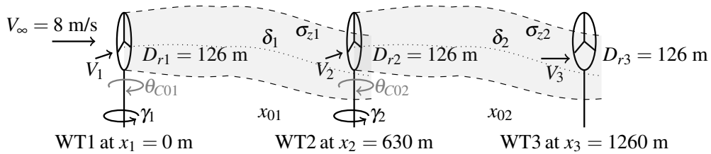
Figure 2.5: Schematic visualization of WRC wind farm optimization, adapted from [Bastankhah and Porté-Agel, 2016].
