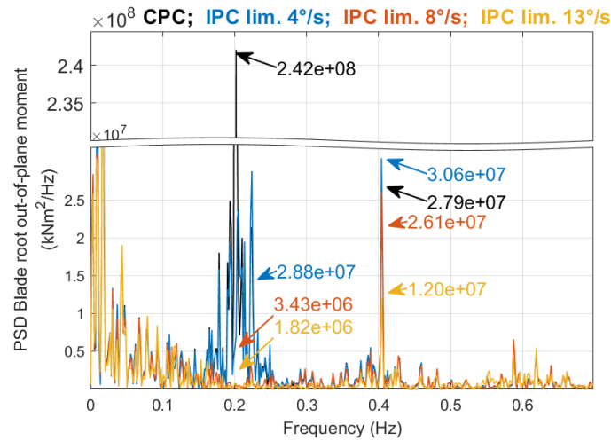
Figure 4.6: Controller comparison: Power Spectral Density of blade root out-of-plane moment of baseline PI (black) with 8^\circ/\text{s} rate limit, IPC with 4^\circ/\text{s} rate limit (blue), 8^\circ/\text{s} rate limit (red), and 13^\circ/\text{s} rate limit (yellow)
