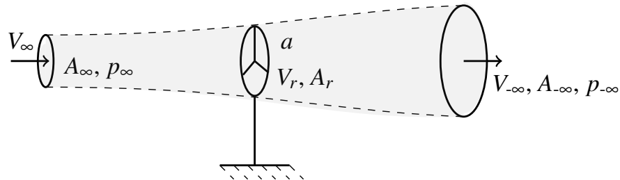
Figure 2.1: Airflow through a wind turbine, modelled as an actuator disk, adapted from [Bianchi et al., 2006].
