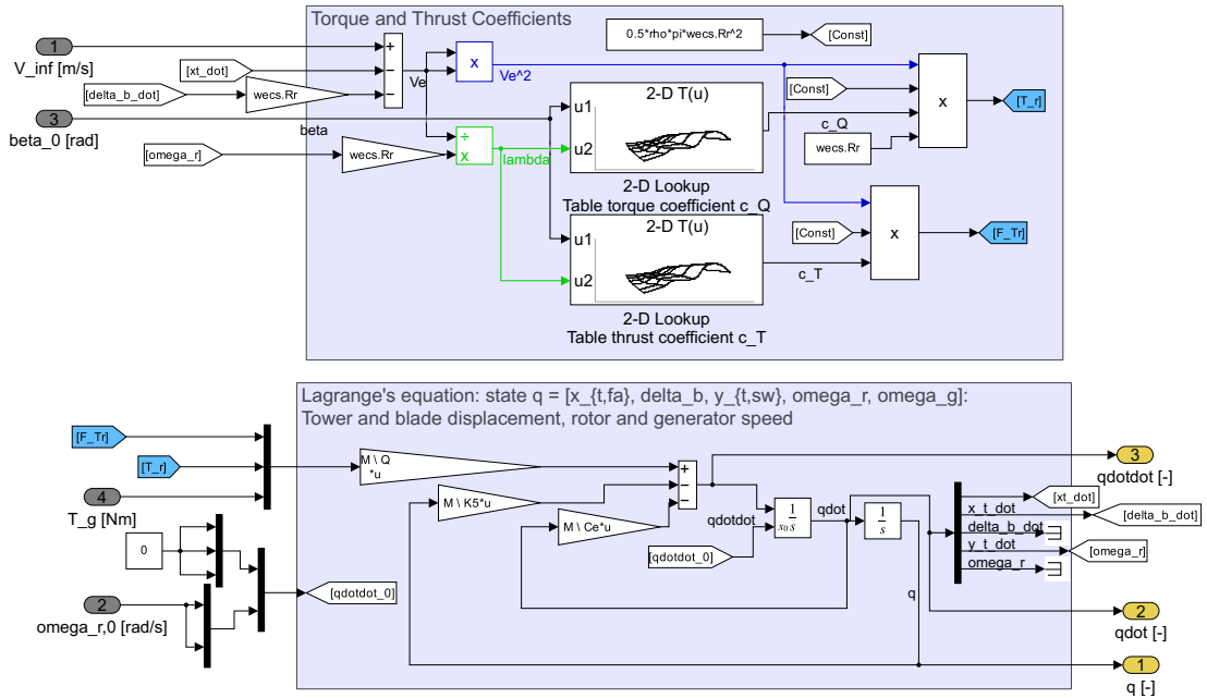
(b) 9th-order model with rotor and generator speed as well as tower and blade displacement states, adapted from [Bianchi et al., 2006].
