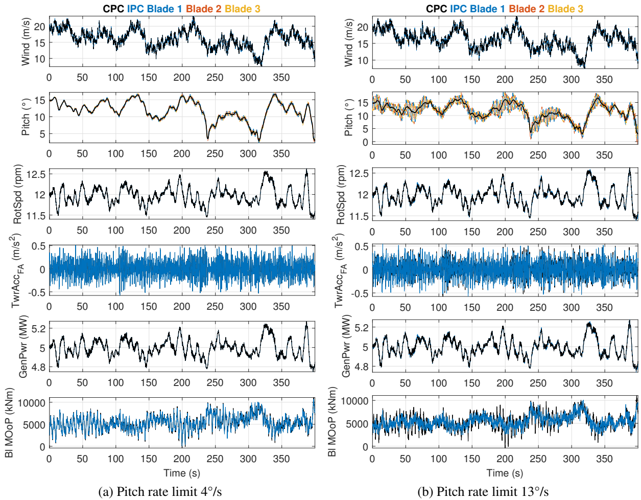
Figure 4.5: Controller comparison: Baseline (black) and IPC PI (blue, red and yellow lines pitch signals, blue all other signals) with different pitch rate limits for turbulent wind (16 m/s mean, IEC turbulence class B (14%)). Rate limits: Low (4°/s) and high (13°/s) for IPC, standard (8°/s) for baseline PI. Displayed signals: wind speed, pitch, states, power, and out-of-plane blade root moments.
