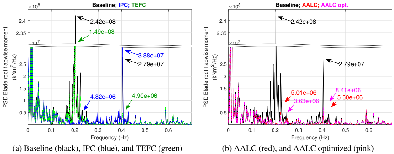
Figure 4.13: Power Spectral Density of optimization set signals, turbulence class A, with mean wind speed 16 m/s.
