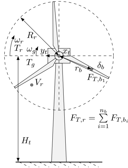
Figure 3.2: Schematic LPV wind turbine model diagram with inputs, states, and parameters.
