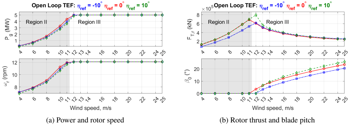
Figure 4.12: TEF open-loop verification, TEF deflection at -10^\circ (blue), 0^\circ (red), and 10^\circ (green).
