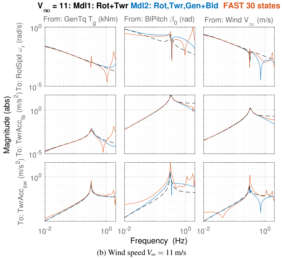
Figure 3.6: Open-loop verification: Frequency response magnitude of linearized FAST and qLPV models for below rated wind speeds. Mdl1 (black dashed line), Mdl2 (blue line), and FAST reference implementation (red line) at frequencies from 0.01 Hz to 2 Hz.
