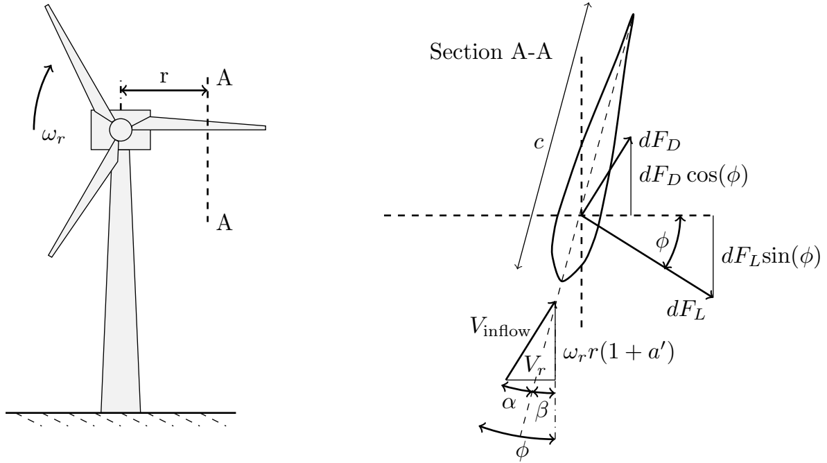
Figure 2.2: Local airflow and forces on a blade element of width dr at radial position r , based on [Hansen, 2015] and adapted from [Weiß, 2016].
