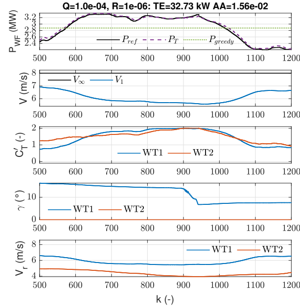
(c) WRC-AIC ( n_u = 3 ): Thrust and yaw controls simultaneously optimized.
