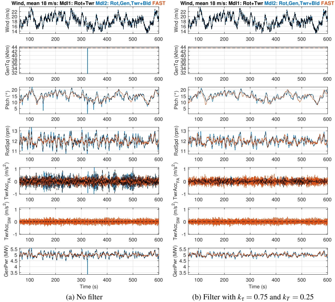
Figure 3.9: Closed-loop model comparison: FAST and qLPV models with PI baseline controller, under turbulent wind, 18 m/s mean, IEC turbulence class B (14%), with and without filter on freestream wind. Mdl1 (black dashed line), Mdl2 (blue line), and FAST reference implementation (red line). Displayed signals: wind, control inputs, rotor speed, tower accelerations, and power.
