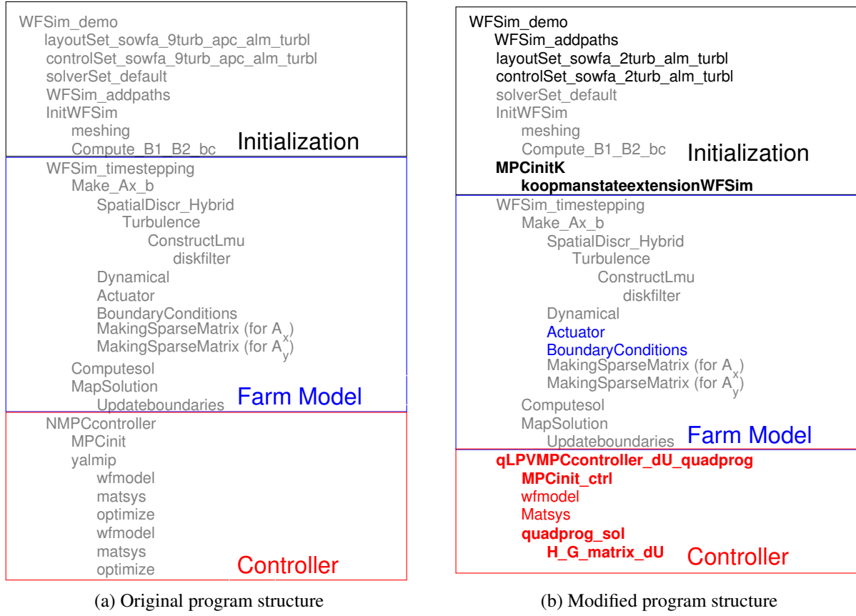
Figure 5.2: WFSim program structure diagram. Initialization, wind farm model, and controller functions are enclosed in black, blue, and red boxes, respectively. Modified functions in (b) are highlighted in black, blue, and red within their respective sections, and functions added for Koopman MPC are indicated in bold.
