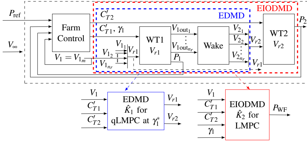
Figure 5.7: Block diagram of WFSim for WRC-AIC with farm control inputs P_{\text{ref}} , P_1 , P_2 , and V_1 = V_{1m} , control signals C_{T1}' , C_{T2}' , \gamma_1 , and freestream wind V_\infty . Local wind speeds upwind and downwind of WT1 are V_{11} \dots V_{1n_r} and V_{1out1} \dots V_{1outn_r} . Wind speeds upwind of WT2 are V_{21} \dots V_{2n_r} . The input to the EDMD model (blue) are V_1, C_{T1}', C_{T2}' with effective wind outputs V_{r1}, V_{r2} . The input to the EIODMD model (red) are V_1, C_{T1}', C_{T2}', \gamma_1 with farm power output P_{\text{WF}} = P_1 + P_2 .
