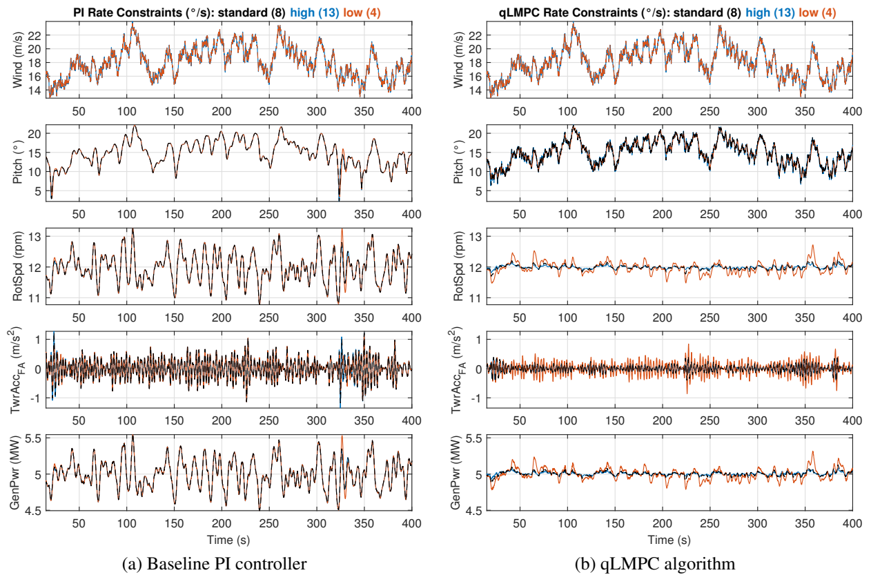
Figure 4.3: Controller comparison: Baseline PI and qLMPC with different pitch rate limits for turbulent wind (18 m/s mean, IEC turbulence class B (14%)). Rate limits: Standard 8^\circ/\text{s} (black line), high 13^\circ/\text{s} (blue line), and low 4^\circ/\text{s} (red line)). Displayed signals: wind speed, pitch, states, and power.
