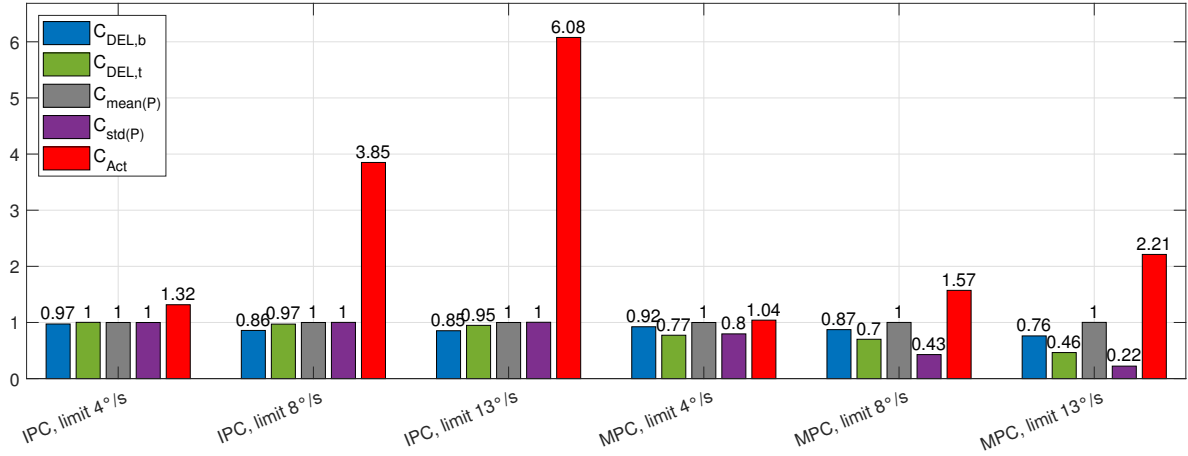
Figure 4.7: Wind turbine controller evaluation criteria qLMPC and IPC for turbulent wind (16 m/s mean, IEC turbulence class B (14%)). Criteria are tower base and blade DELS, power mean and standard deviation, and pitch actuator power.
