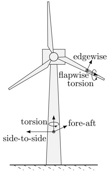
Figure 3.1: Schematic wind turbine diagram of tower and blade movements.
