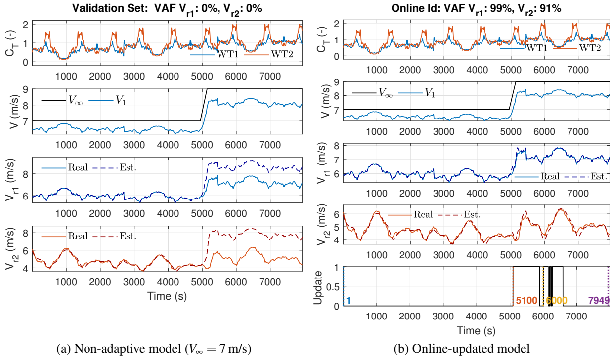
Figure 5.4: Open-loop identification comparison during a wind speed step at t = 5000 s. Subplots (top to bottom): thrust C_T ; wind speeds V_\infty (black) and V_1 (blue); and real vs. estimated effective wind V_{r1} , V_{r2} . Bottom plot in (b) shows the update signal (black). WT1/WT2 signals are blue/red; dashed lines denote estimates.
