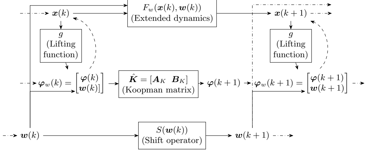
Figure 2.9: Block diagram of the nonlinear system, approximated lifting function, shift operator, and Koopman matrix propagation for a forced system (adapted from [Proctor et al., 2018])
