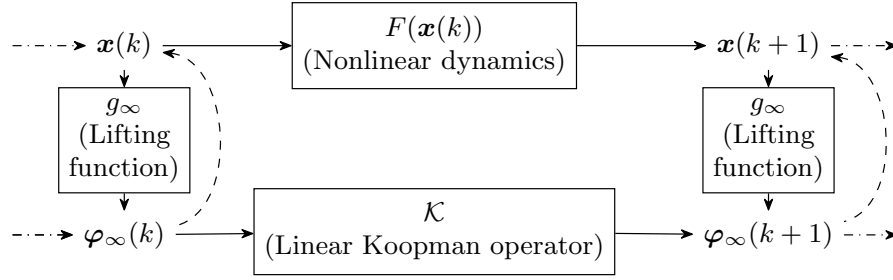
Figure 2.8: Block diagram of the nonlinear system, lifting function, and linear Koopman operator propagation for an unforced system (adapted from [Brunton et al., 2016]).
