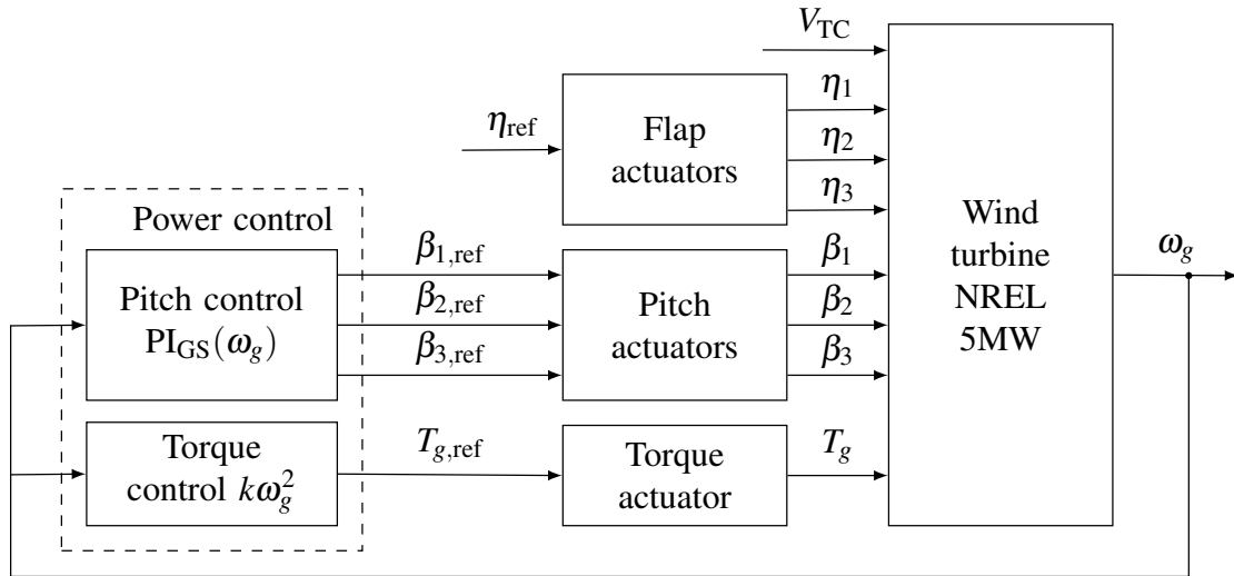
Figure 4.10: Block diagram for open-loop TEF verification tests with baseline power control in closed loop and open-loop collective TEF control inputs.
