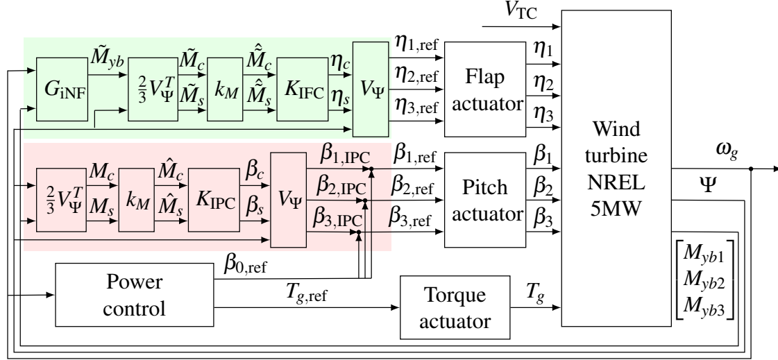
Figure 4.11: Block diagram for closed-loop verification tests with baseline power control, individual pitch (highlighted in red) and TEF (highlighted in green) closed loop control.
