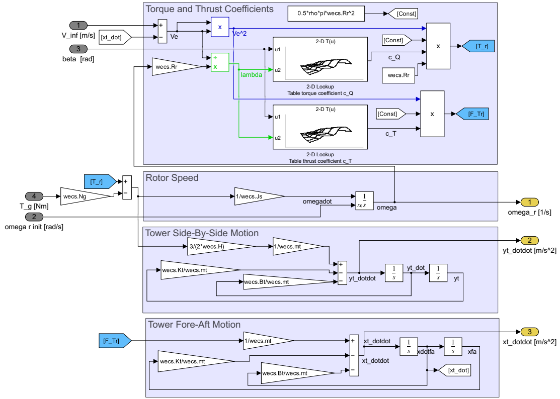
(a) 5th-order model with rotor speed and tower displacement states, adapted from [Mulders et al., 2020a].
