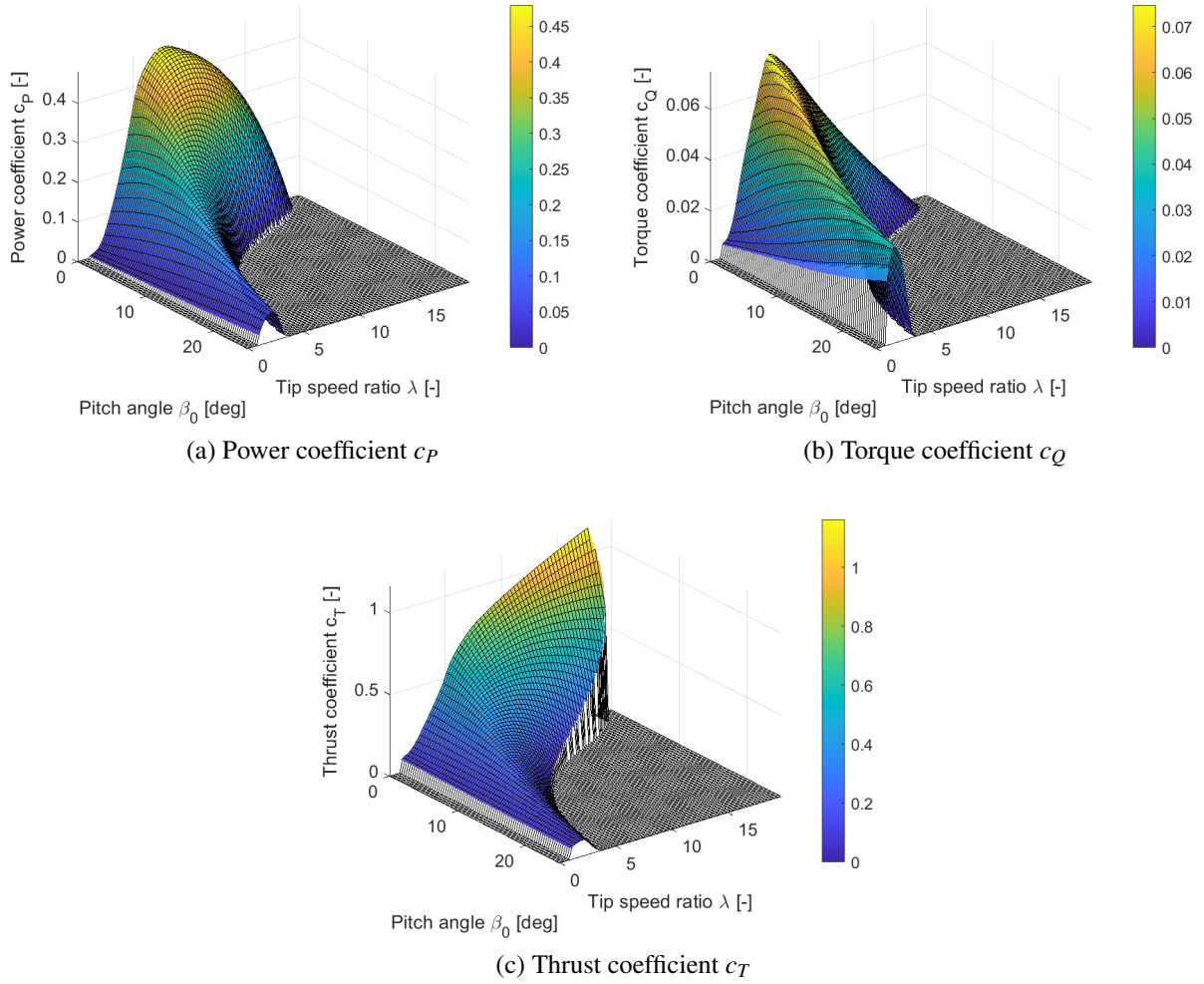
Figure 3.3: Aerodynamic power, torque and thrust coefficient surfaces with respect to blade pitch angle and tip speed ratio for the NREL 5MW model.
