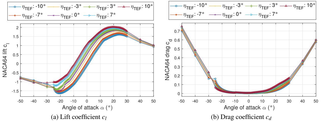
Figure 4.9: Lift and drag coefficients at different TEF angles \eta_{TEF} and different blade angles of attack \alpha .
