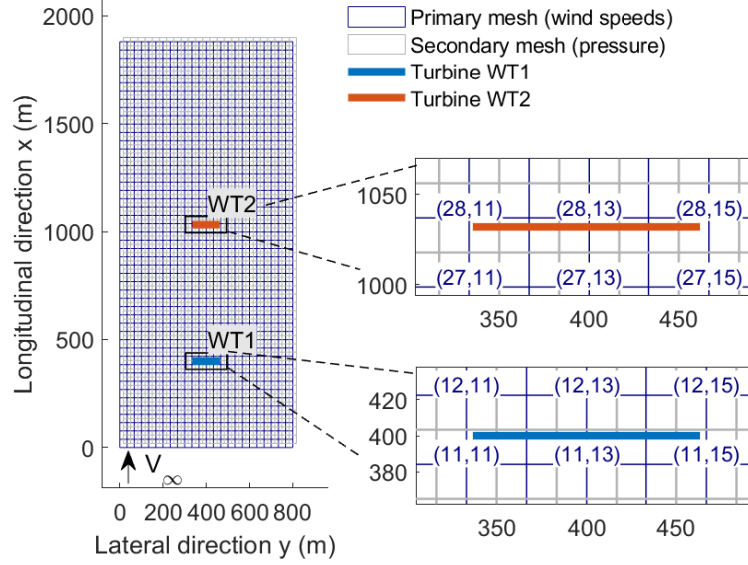
Figure 5.1: WFSim mesh setup for the two-turbine wind farm. The primary mesh (blue) is used for wind speed calculations, and the secondary mesh (gray) for pressure. WT1 (upstream) and WT2 (downstream) are shown as blue and red bars, respectively. Zoomed-in areas show primary grid point indices.
