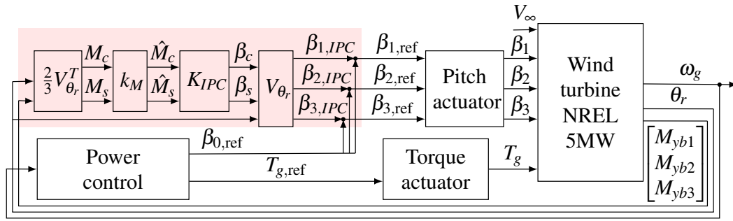
Figure 4.4: Block diagram of the closed-loop wind turbine control structure with IPC PI (highlighted in red) added to the baseline PI controller.
