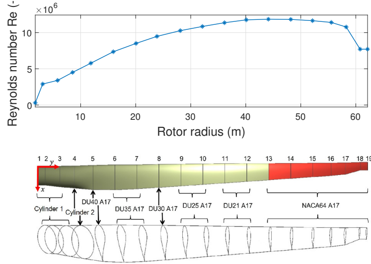
Figure 4.8: Span-wise distribution of Reynolds numbers Re at wind speed V_\infty = 12 m/s (from OpenFAST simulation) and blade geometry with cylinder, DU40, DU35, DU30, DU25, DU21 and NACA64 profiles with TEF location covering the NACA64 section marked in red.
