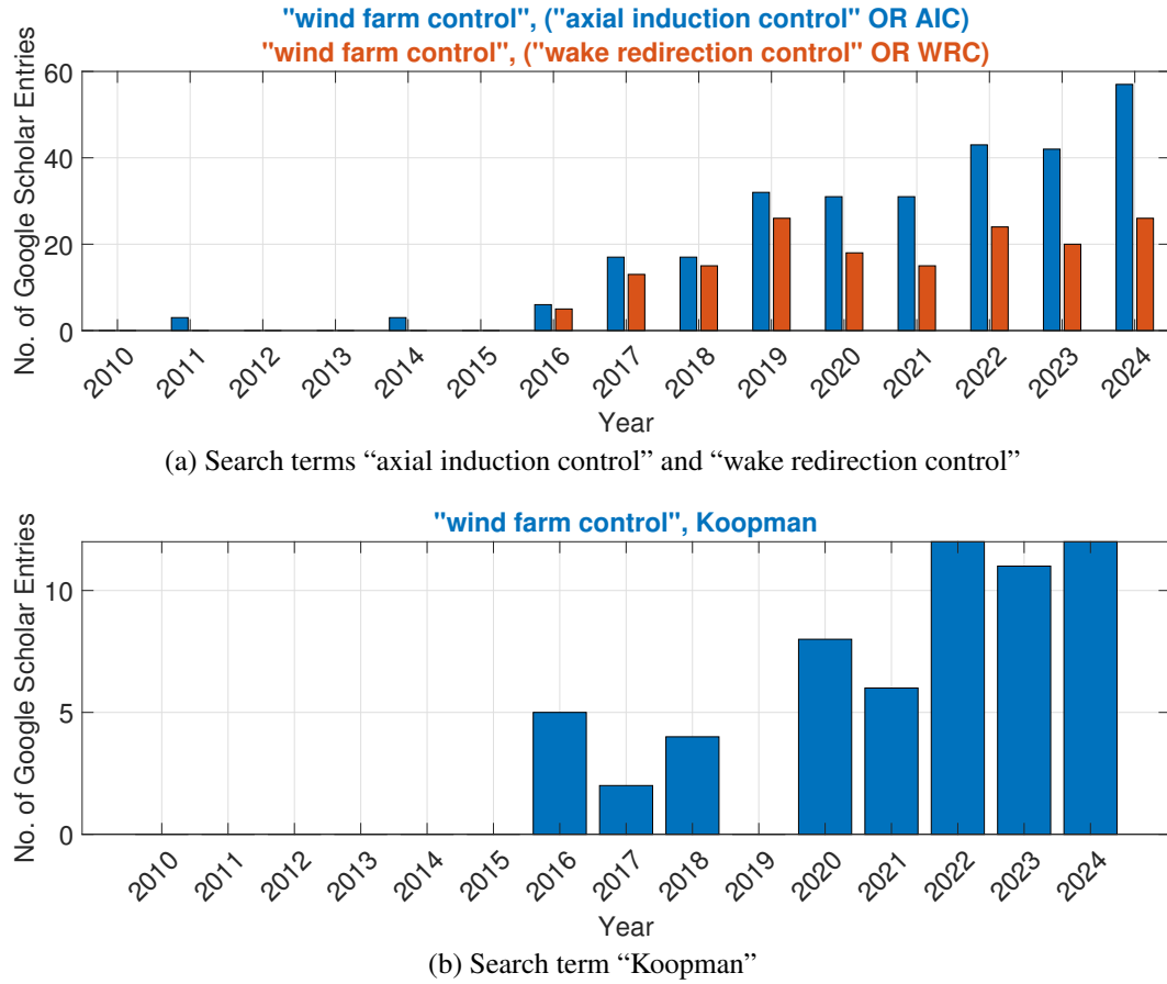
Figure 1.3: Number of Google Scholar results by year for the search term “wind farm control” and different additional search terms
