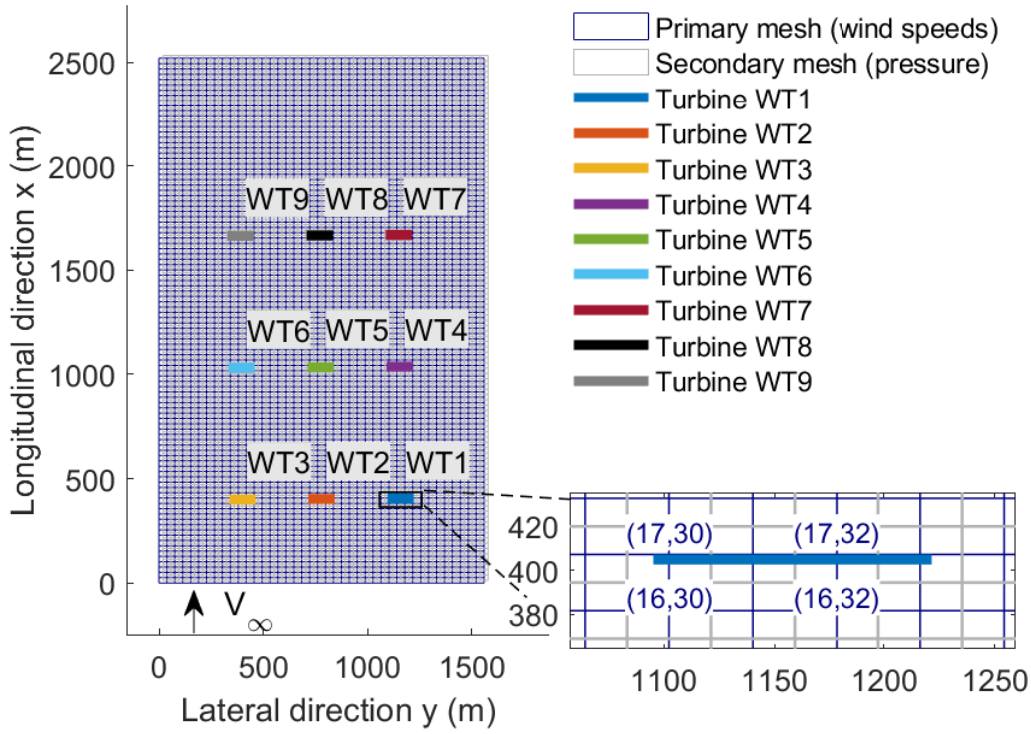
Figure 2.6: WFSim mesh setup for a nine-turbine wind farm. The primary mesh (blue) is used for wind speed calculations, and the secondary mesh (gray) for pressure. Turbines are shown as colored bars. Zoomed-in area around WT1 shows primary grid point indices.
