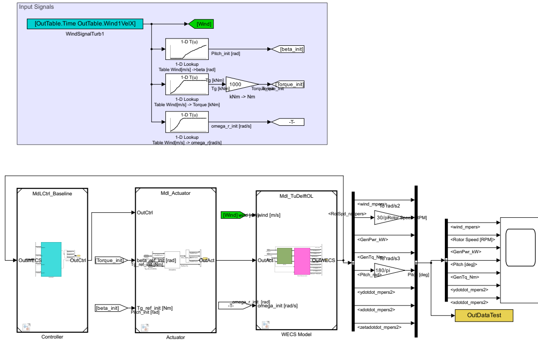
Figure 3.4: Simulink model for closed loop verification including controller, actuator, and WECS model. The wind is created with the FASTTool and used for the initialization of the generator torque, the blade pitch and the rotor speed.
