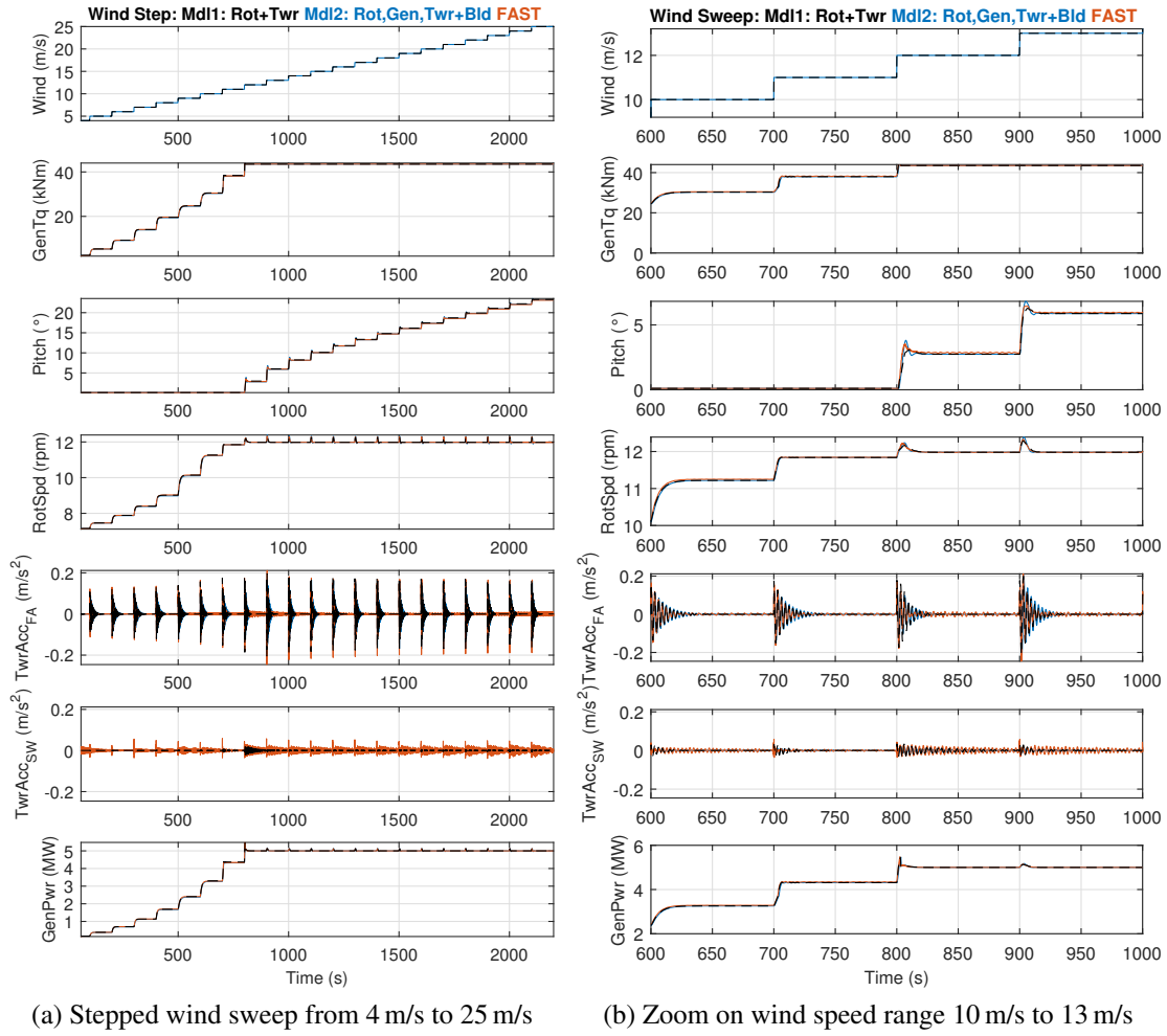
Figure 3.8: Closed-loop verification: FAST and qLPV models simulated in closed loop with the PI baseline controller with a stepped wind sweep from 4 m/s to 25 m/s. Mdl1 (black dashed line), Mdl2 (blue line), and FAST reference implementation (red line). Displayed signals: wind, control inputs, rotor speed, tower accelerations, and power.
