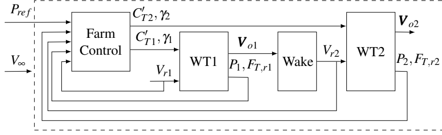
Figure 2.7: Block diagram of closed-loop wind farm control in WFSim
