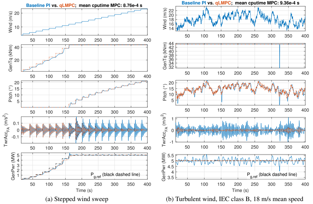
Figure 4.2: Controller comparison: qLPV model with baseline PI controller vs. qLMPC for stepped wind sweep and turbulent wind (18 m/s mean, IEC turbulence class B (14%)). PI control (blue line), qLMPC (red line) and power reference (black dashed line). Displayed signals: wind speed, control inputs, tower fore-aft accelerations, and power output.
