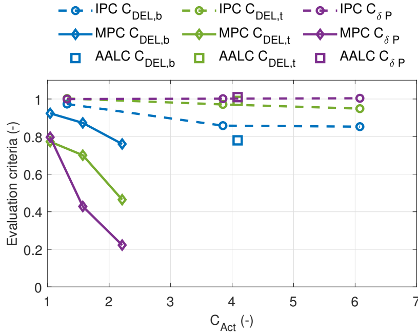
Figure 4.14: Evaluation criteria for qLMPC, IPC, and AALC for turbulent wind (16 m/s mean, IEC turbulence class B (14%)). Criteria are tower base and blade DELs, power mean and standard deviation, and actuator power.
