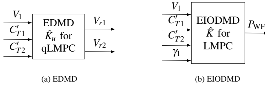
Figure 2.10: Inputs and outputs of the EDMD and EIODMD models with lifted states \varphi based on effective wind speeds V_{r1} and V_{r2} .
