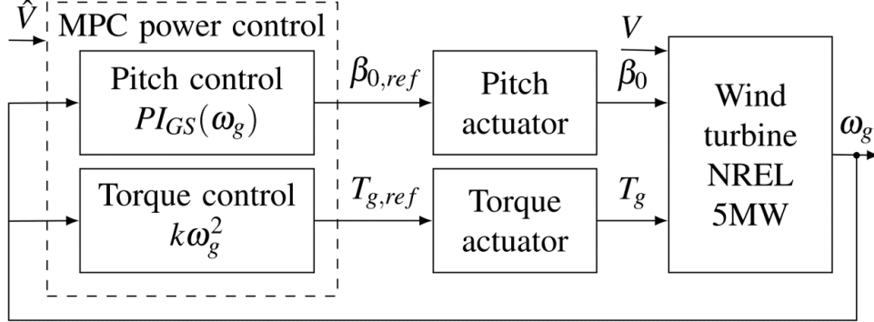
Figure 4.1: Block diagram of the closed-loop wind turbine control structure with qLMPC (dashed box) replacing the baseline PI controller (solid line)
