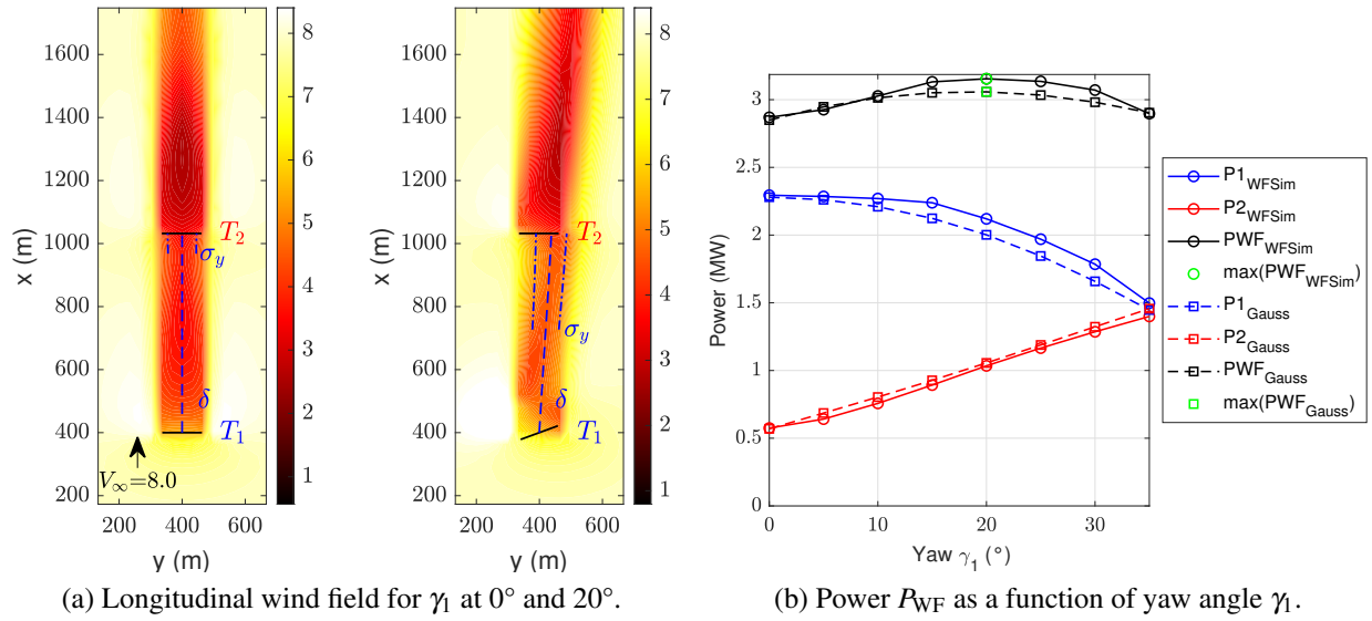
Figure 5.8: Open-loop validation of the Gaussian wake model against WFSim: (a) steady-state longitudinal wind field with Gaussian wake centerline \delta and expansion \sigma_y as blue dashed and dash-dotted lines; (b) power output comparison where WFSim results are marked with circles and the Gaussian model with squares: WT1 (blue), WT2 (red), total wind farm (black), and maximum power point (green)
