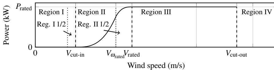
Figure 2.3: Power output curve in Regions I to IV, based on the control region definitions for the NREL 5-MW reference turbine in [Jonkman et al., 2009].
