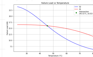
FAILURE LOAD VS TEMPERATURE COMPARISON BETWEEN JOINT SOLUTIONS
