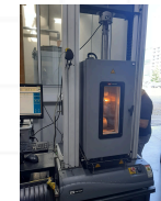
TENSILE TESTING WITH ENVIRONMENTAL CHAMBER
