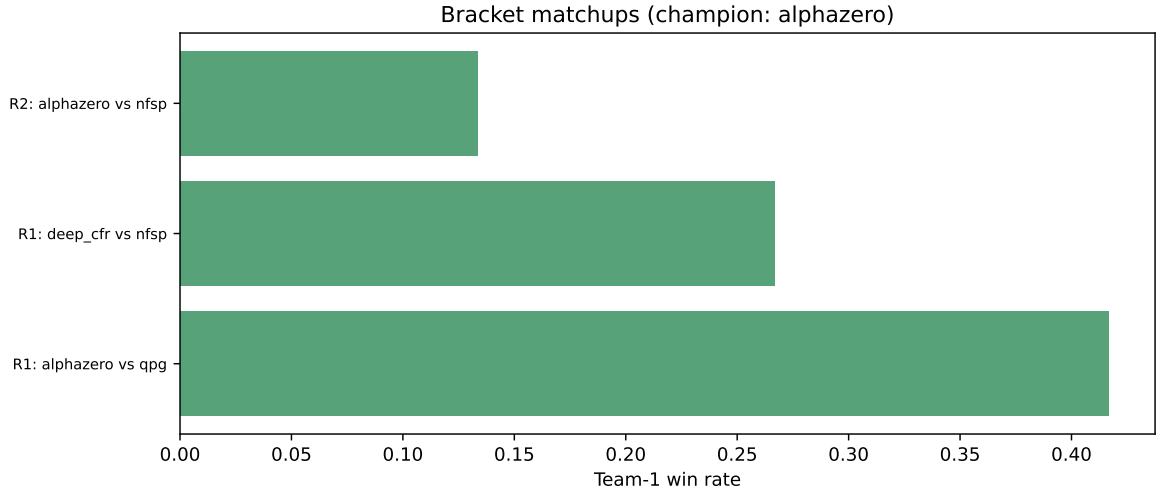
Figure 3: Head-to-head bracket results.
