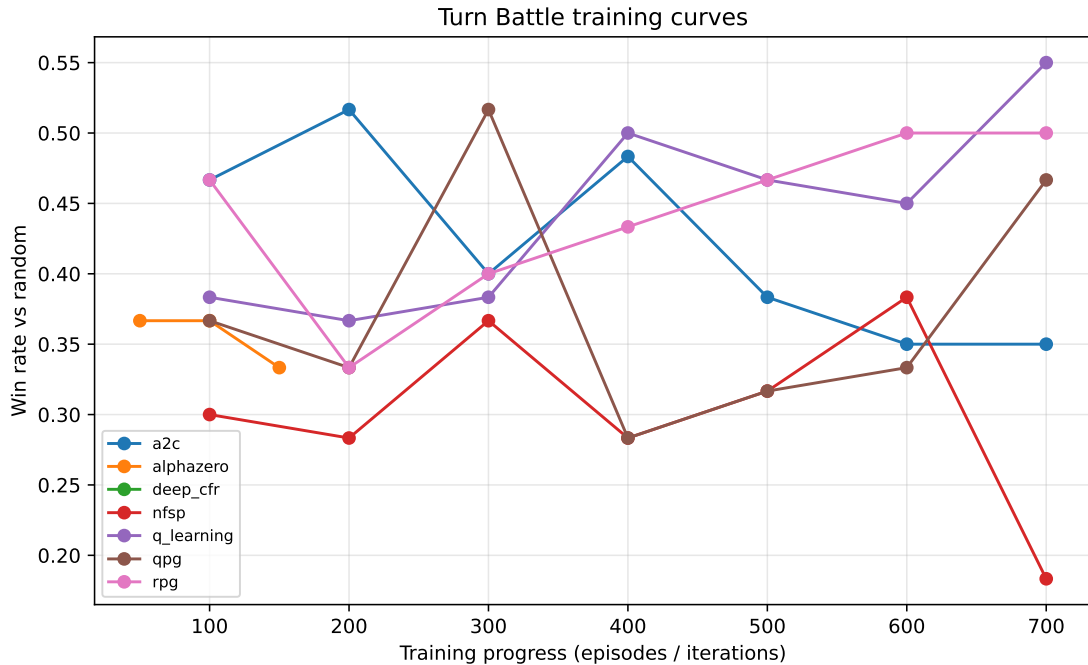
Figure 1: Training progress per algorithm.
