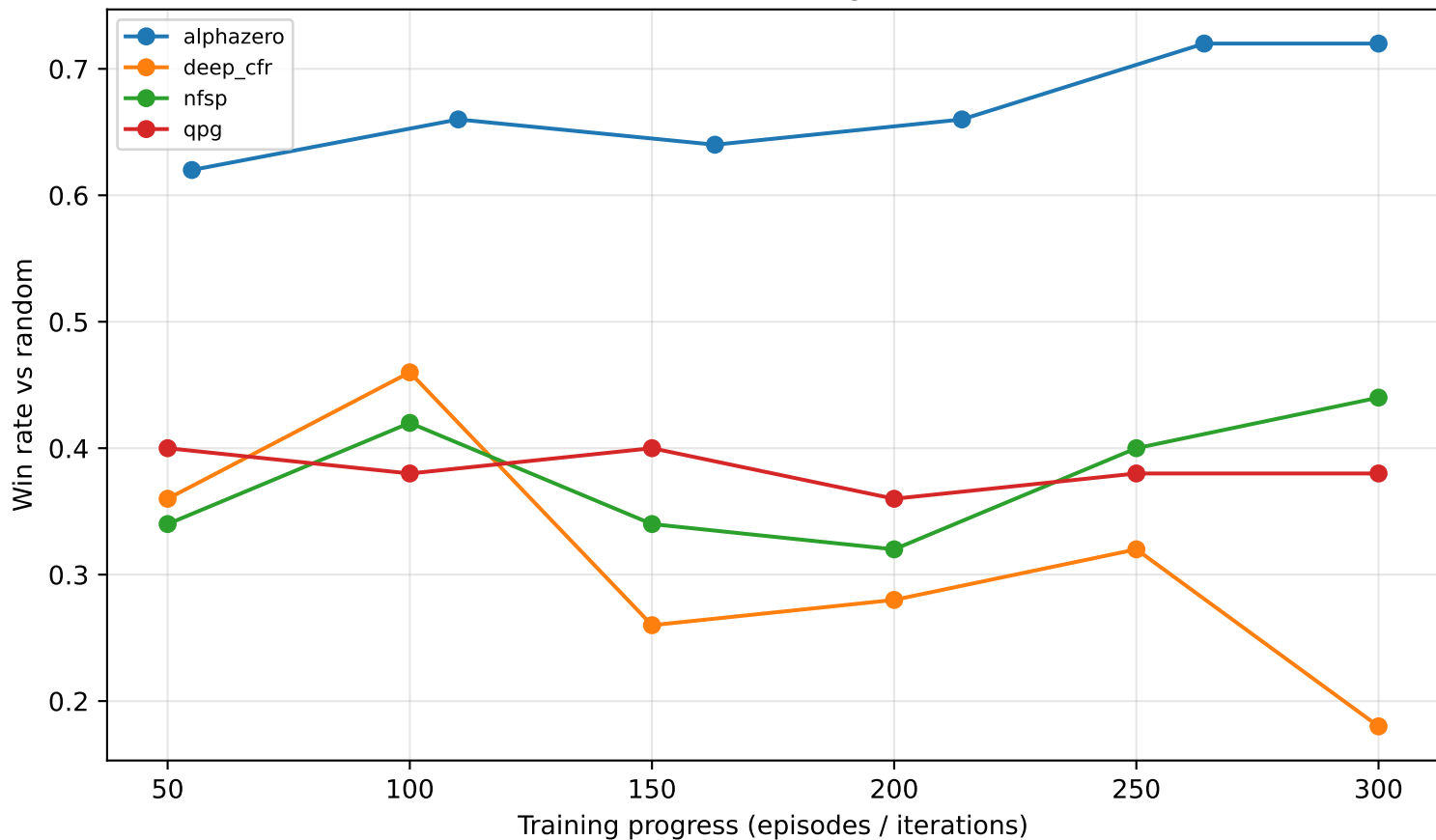
Turn Battle training curves
