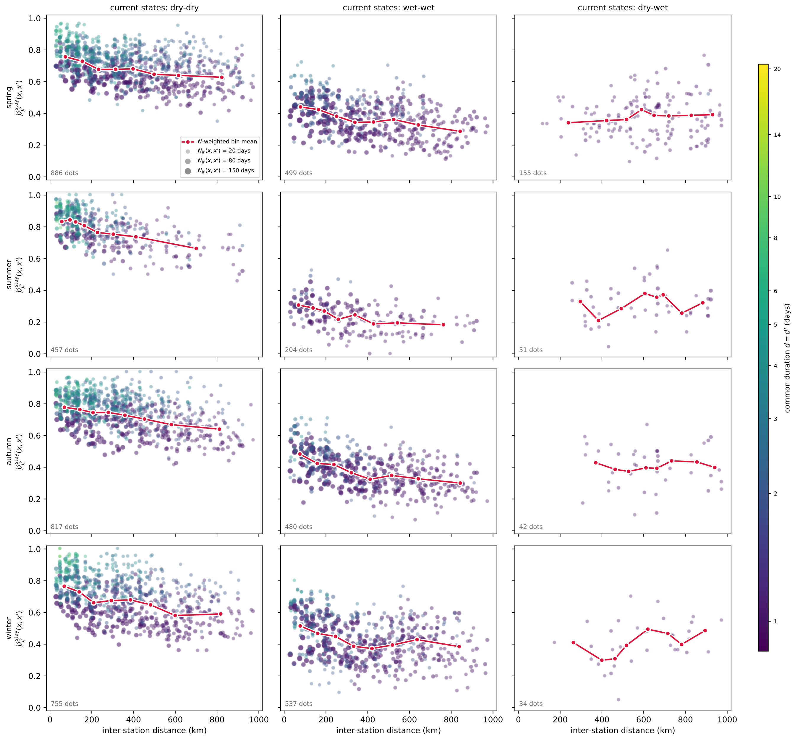
\hat{p}_{jj'}^{\text{stay}}(x, x') against distance, simulated data from fitted model
