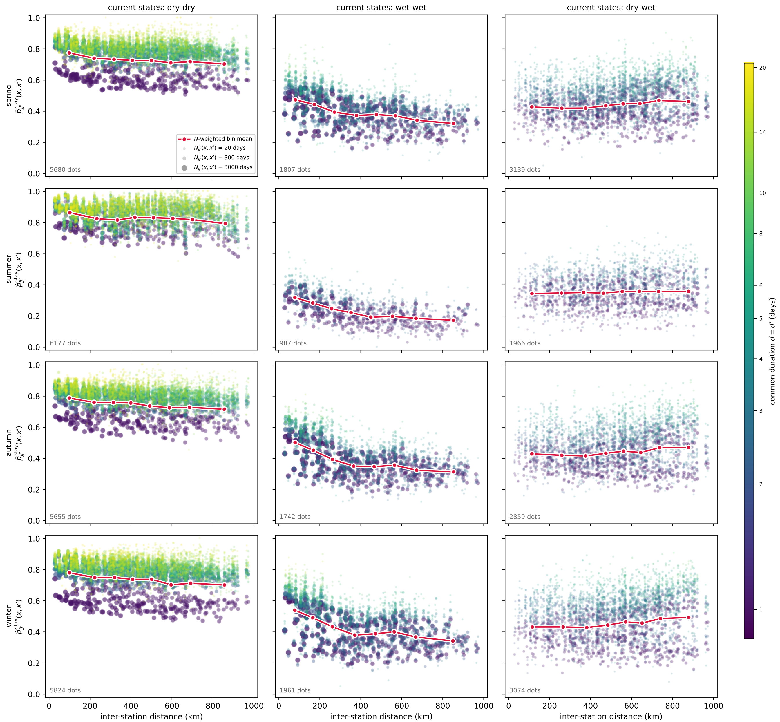
\hat{\rho}_{jj'}^{\text{stay}}(x, x') against distance, simulated data from fitted model, 1025 years
