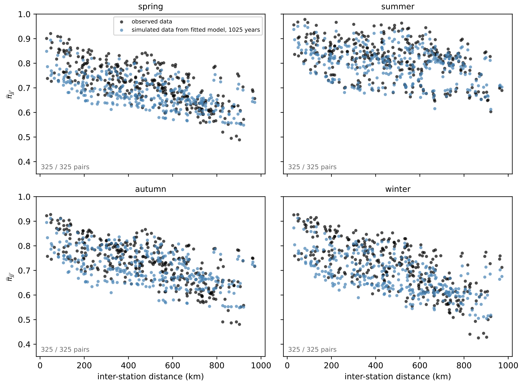
Rain-state agreement \hat{\pi}_{jj'} against distance, observed data vs simulated data from fitted model, 1025 years
