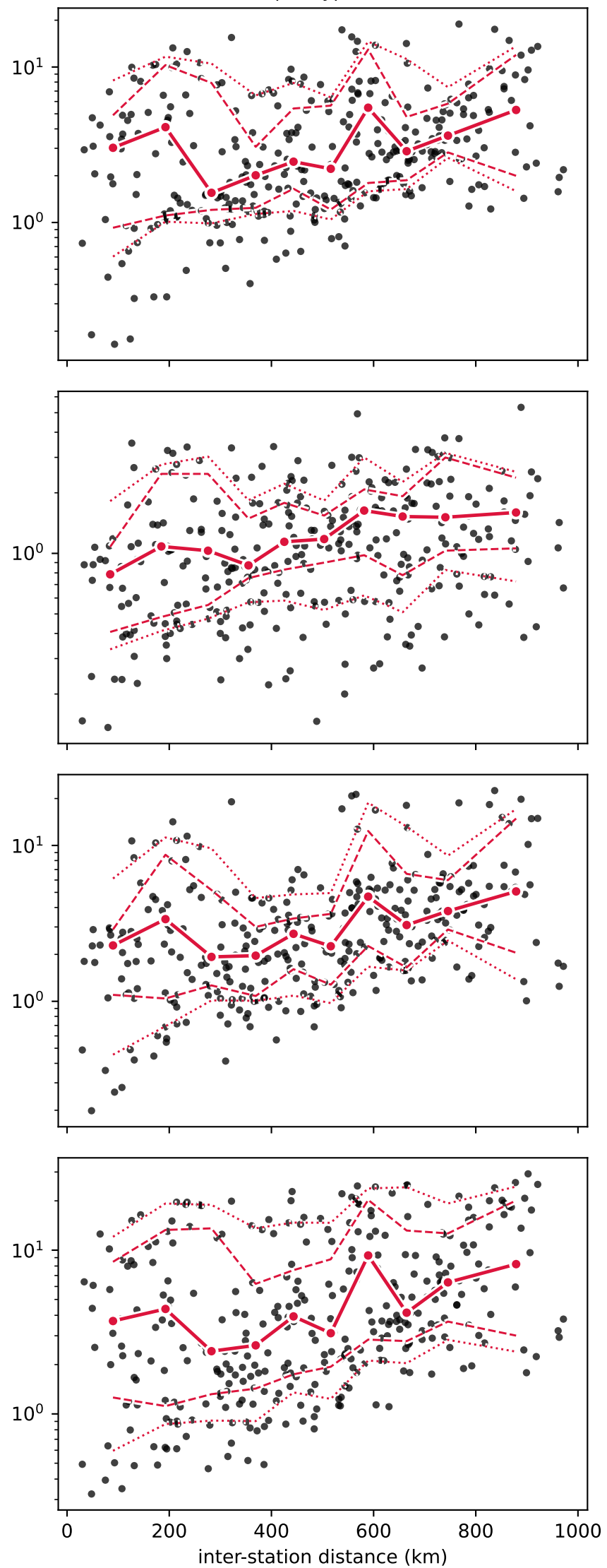
current spell types: wet-wet
