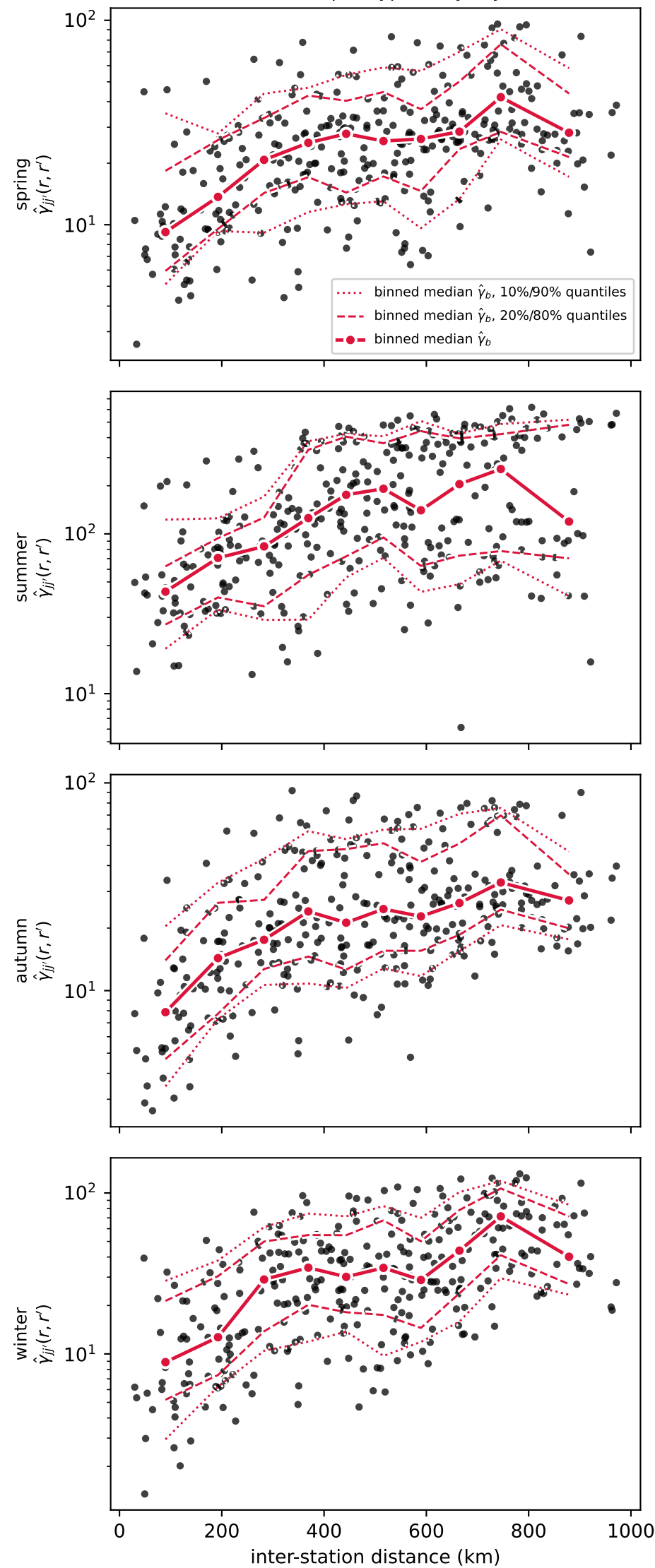
current spell types: dry-dry
