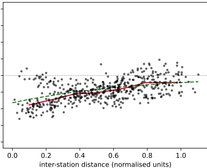
current states: dry-wet
