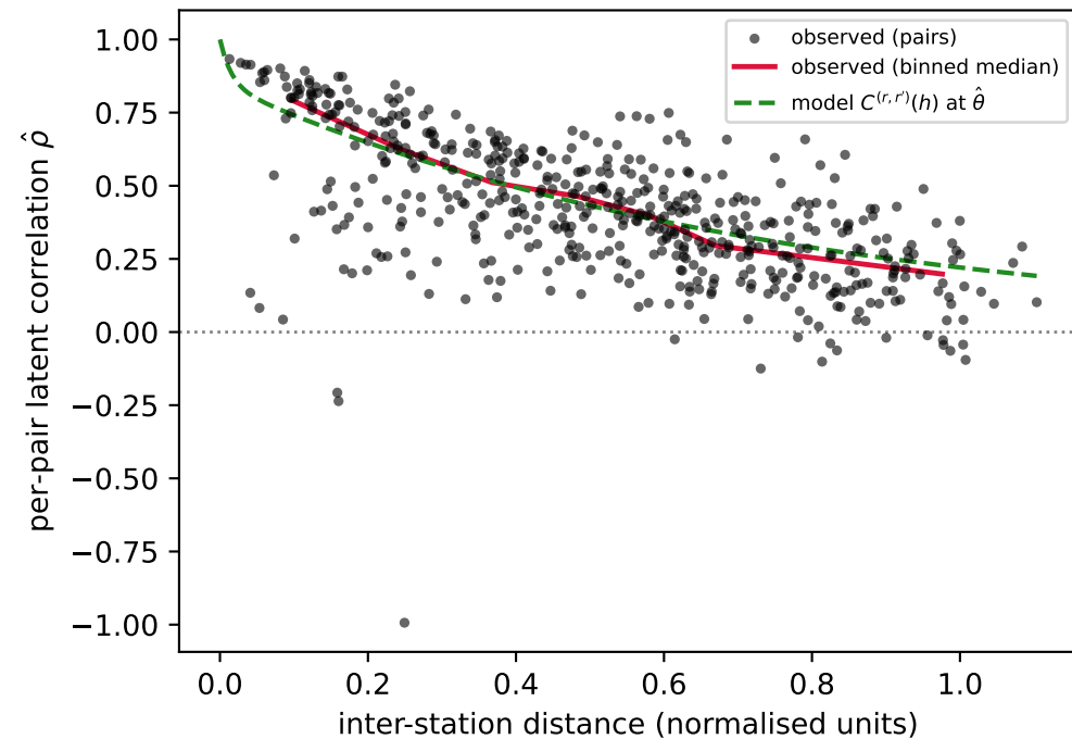
current states: dry-dry
