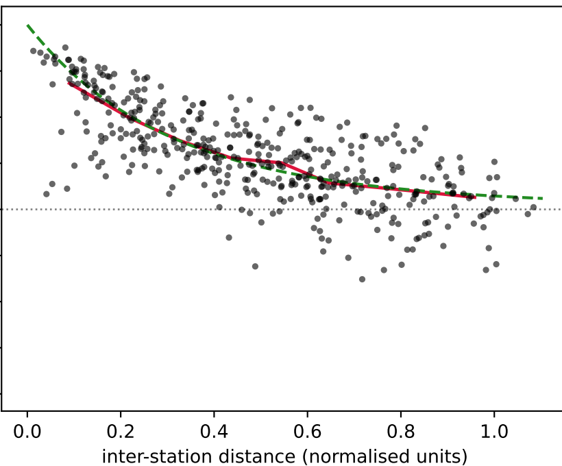
current states: wet-wet
