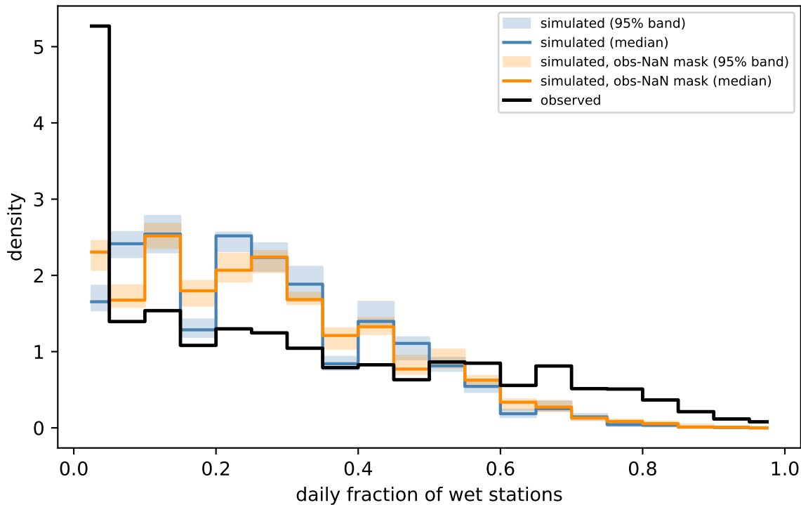
Wet fraction: unmasked vs obs-NaN-masked simulations
