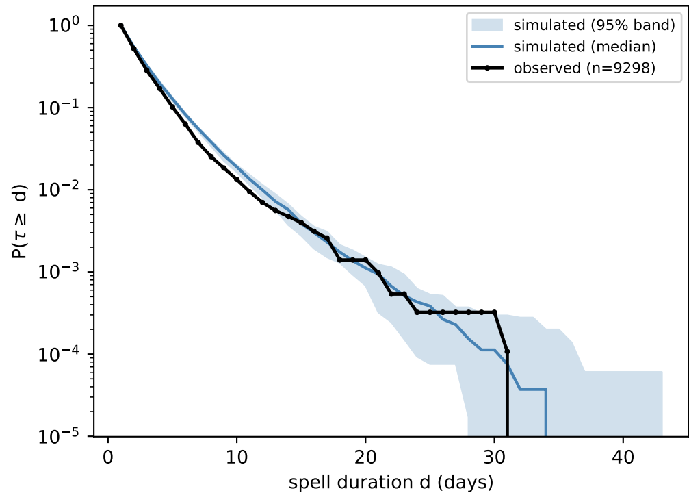
wet spells (complete, pooled over stations)
