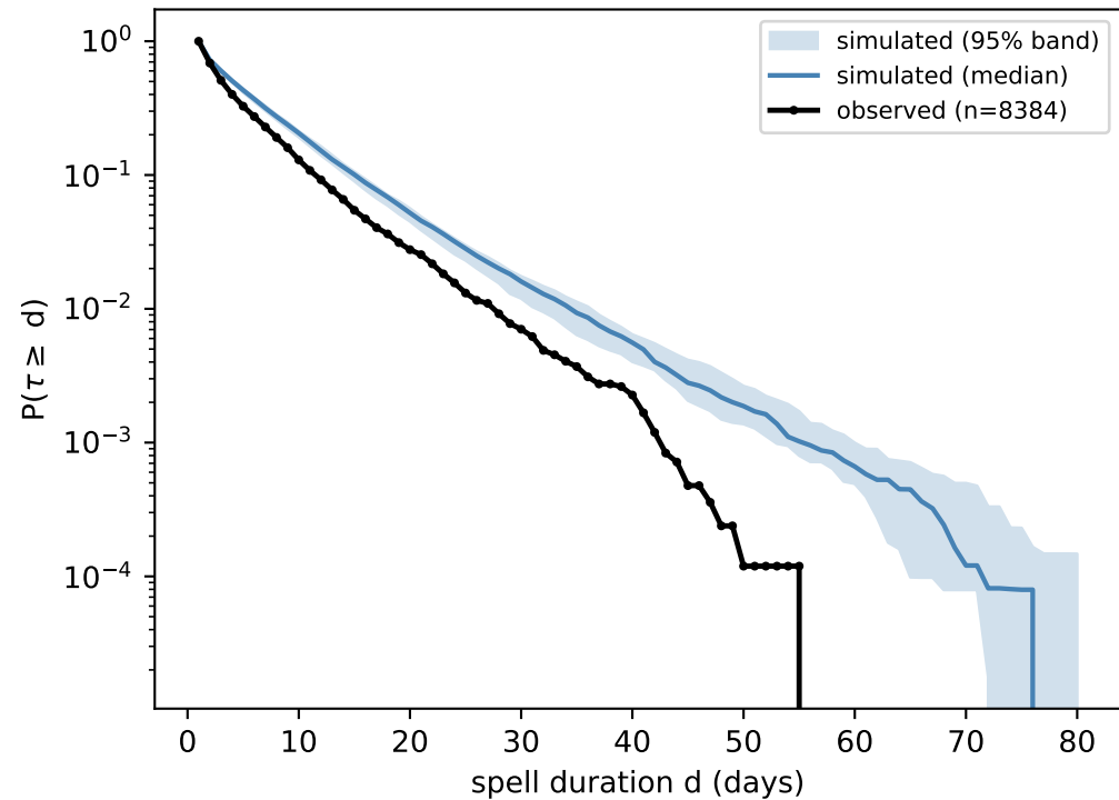
dry spells (complete, pooled over stations)
