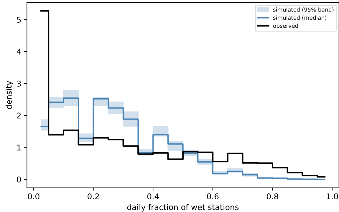
Distribution of the daily wet fraction
