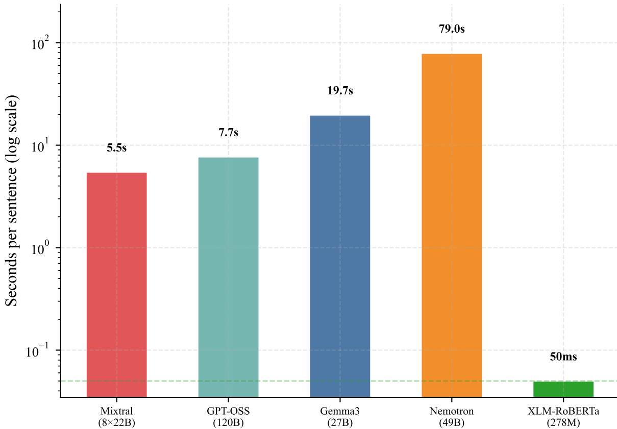
(a) Inference Time per Sentence
