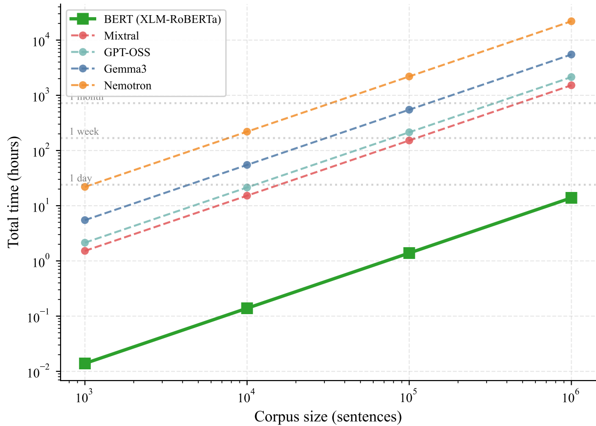
(b) Scaling Projection
