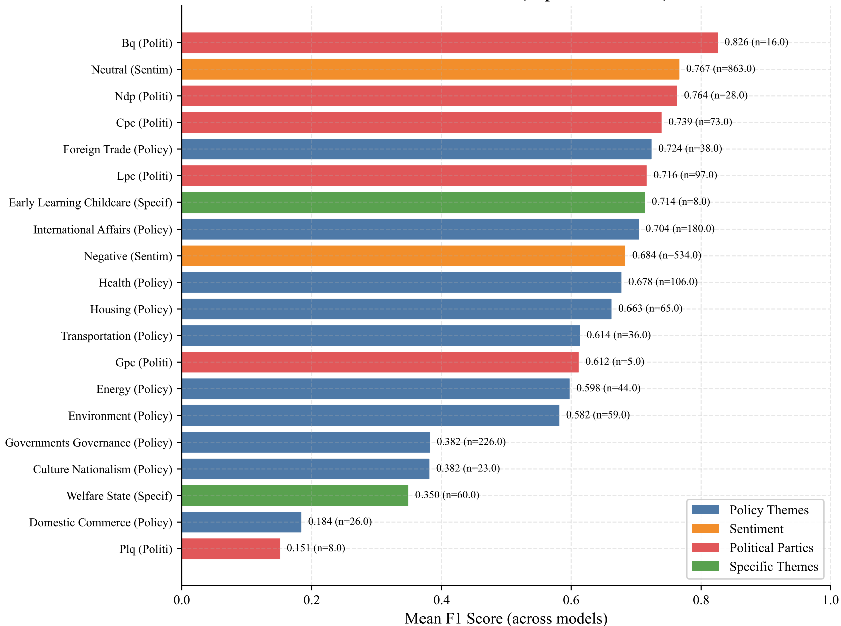
Per-Class Performance (Top 15 + Bottom 5)
