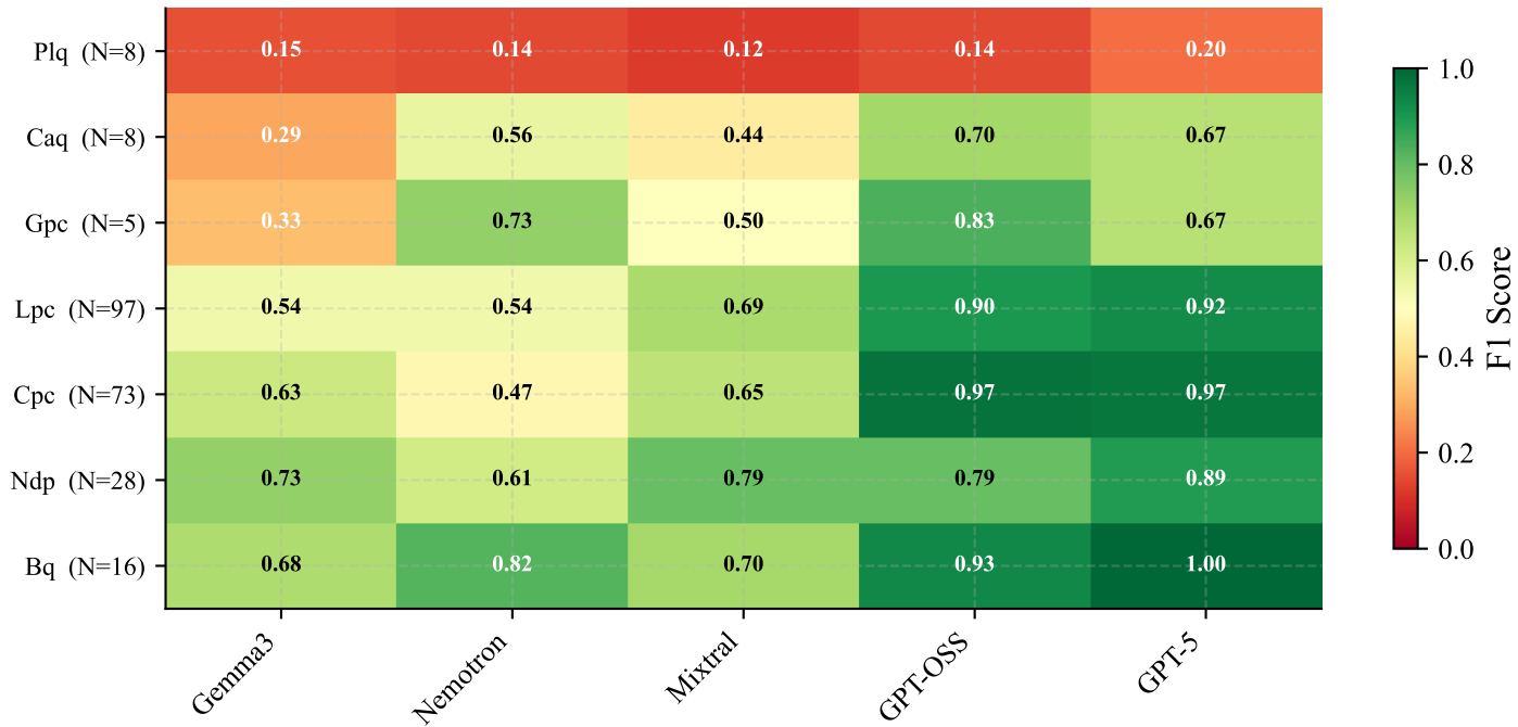
Per-Class F1 Scores — Political Parties
