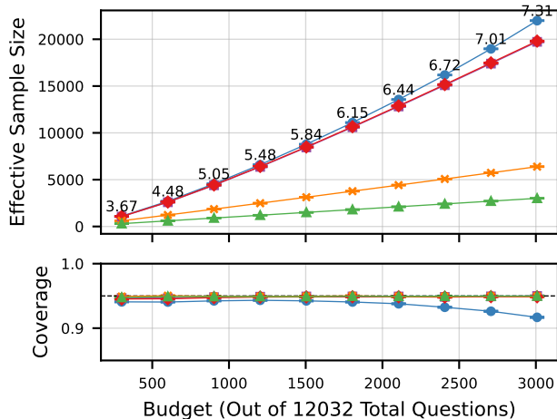
MMLU-Pro
