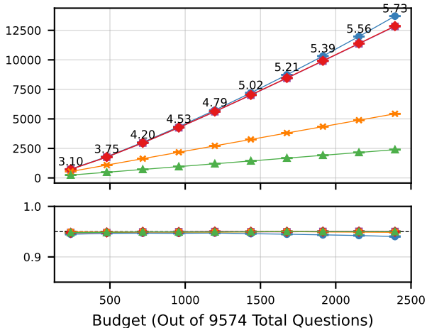
BBH+GPQA+IFEval+MATH+MuSR
